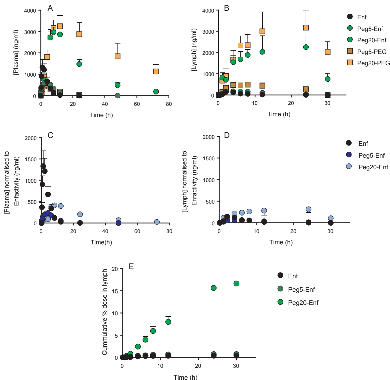
Fig. 3. Concentration versus time profiles of unmodified and PEGylated Enf in plasma and lymph after SC administration of 1.2 mg/kg Enf equivalents to rats. Panels represent (A) plasma concentration vs time profiles of Enf constructs after assaying for Enf (green circles) and PEG (brown squares); (B) lymph concentration vs time profiles of Enf constructs after assaying for Enf (green circles) and PEG (brown squares); (C) plasma concentration vs time profiles of Enf constructs (by assaying for Enf) after normalising concentrations to unmodified Enf activity; (D) lymph concentration vs time profiles of Enf constructs (by assaying for Enf) after normalising concentrations to unmodified Enf activity; (E) cumulative % recovery of the SC doses in thoracic duct lymph over 30 h. Data represents mean \pm s.e.m. (n = 4). (For interpretation of the references to colour in this figure legend, the reader is referred to the web version of this article.)
