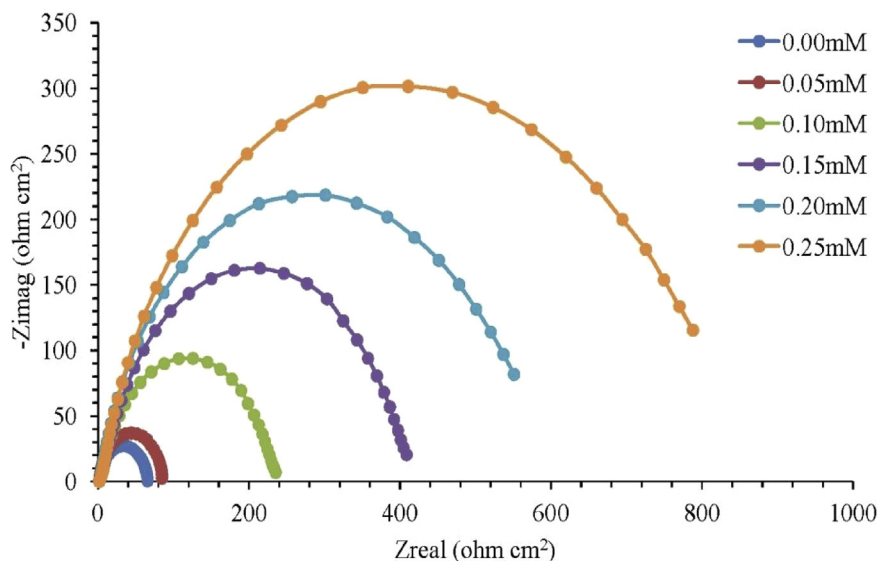
Fig. 4. Mild steel Nyquist plot in 1M \text{H}_2\text{SO}_4 at 30 °C for varying OGCI concentrations [86].
