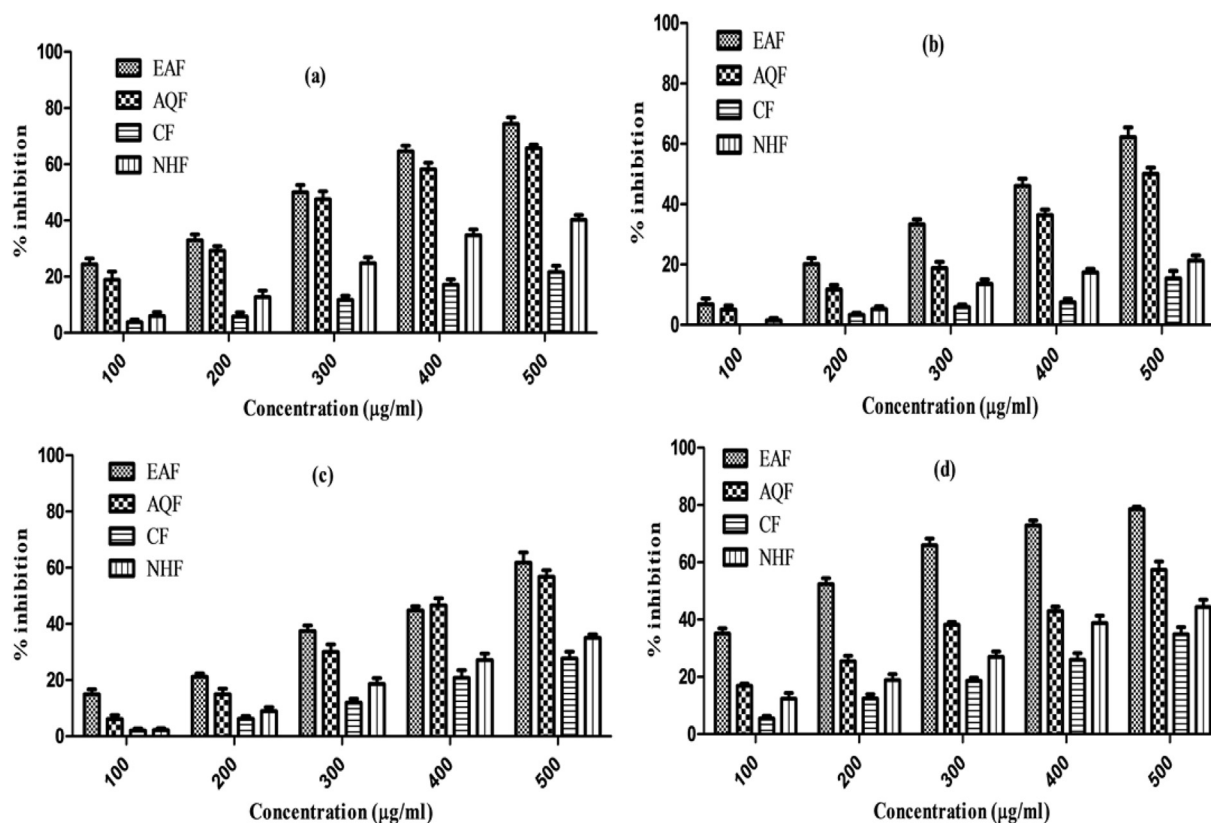
Fig. 5. Alfa glucosidase activity of different samples on (a) Soxhlet extract, (b) Maceration extract, (c) Ultrasound extract and (d) Microwave assistant extract. Each value is presented as mean \pm standard deviation ( n = 3 ).
