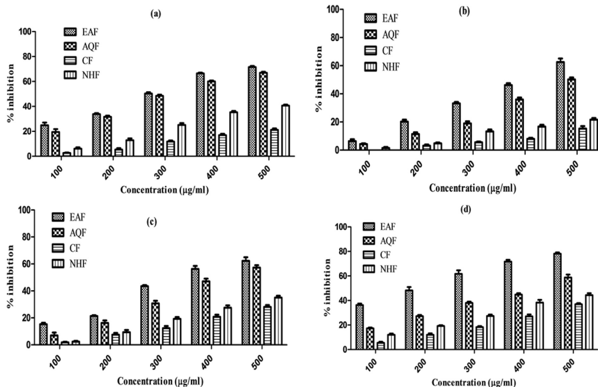
Fig. 4. Alfa amylase activity of different samples on (a) Soxhlet extract, (b) Maceration extract, (c) Ultrasound extract and (d) Microwave assistant extract. Each value is presented as mean \pm standard deviation ( n = 3 ).
