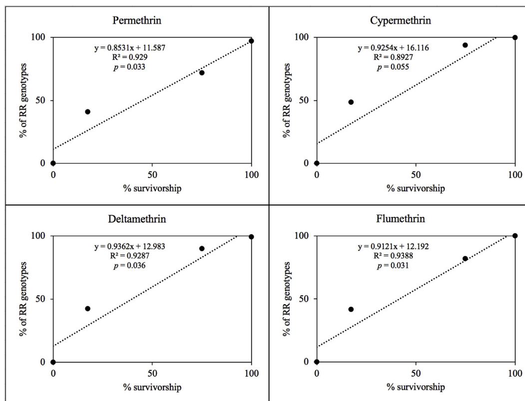
Fig. 6. Linear regressions of R. microplus of susceptible (Deutsch) and resistant strains (Santa Luiza, El Zamora and Yucatan), showing the relationship between the proportion of individuals carrying the mutations in homozygosis and the larval packet test survivorship using permethrin, cypermethrin, deltamethrin and flumethrin.
