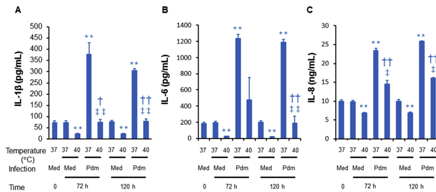
Fig. 7. The levels of IL-1β, IL-6 or IL-8 in the cell supernatants in cells cultured before (time 0) or at 72 h or 120 h after infection with sham (med) or the A/H1N1 pdm 2009 virus (pdm) and culture at 37 °C or 40 °C. The results are expressed as the means ± SEM of three tracheae. Significant differences from uninfected cells cultured at 37 °C are indicated by ** p < 0.01 . Significant differences from uninfected cells cultured at 40 °C are indicated by † p < 0.05 and †† p < 0.01 . Significant differences from infected cells cultured at 37 °C are indicated by ‡ p < 0.05 and ‡‡ p < 0.01 .
