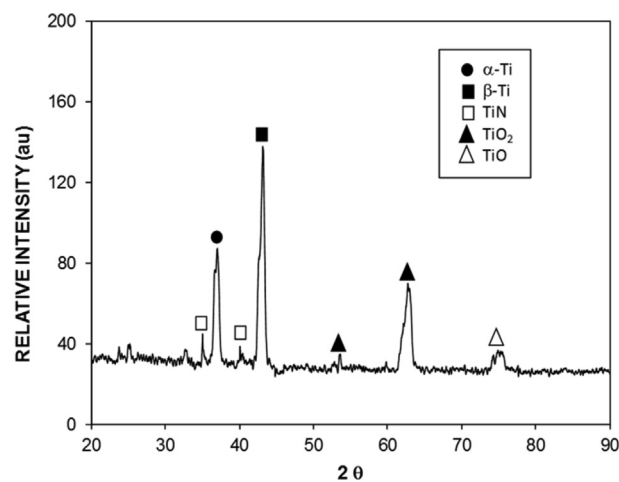
Fig. 3. X-ray diffractogram of laser treated surface.
