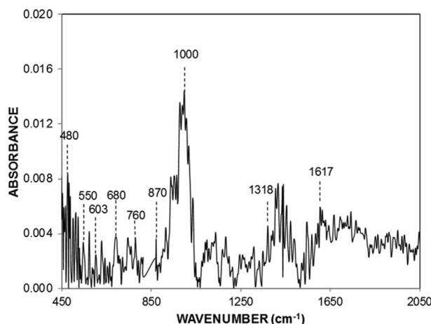
Fig. 5. FTIR data of laser processed surface.
