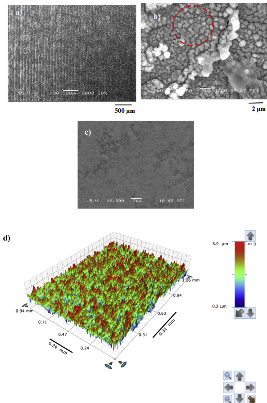
Fig. 1. SEM micrographs of laser treated and as received, and 3D optical image of the laser treated surface: a) SEM micrograph showing regular scanning tracks, b) micro/nano size surface texture (dotted red circle), c) as received surface, and d) 3D optical image of surface topology of laser treated surface.
