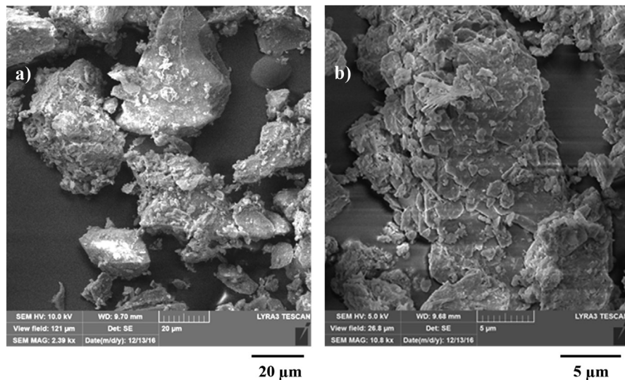
Fig. 8. SEM micrographs of dust particles: different shapes and sizes, b) small size dust attaching at dust particles surface.
