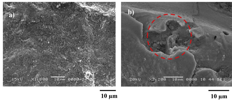
Fig. 12. SEM micrographs of surfaces after removal of dried solution from surface by desalinated water jet: a) laser processed surface, and b) as received surface and shallow pit site is evident (marked in a dotted circle).
