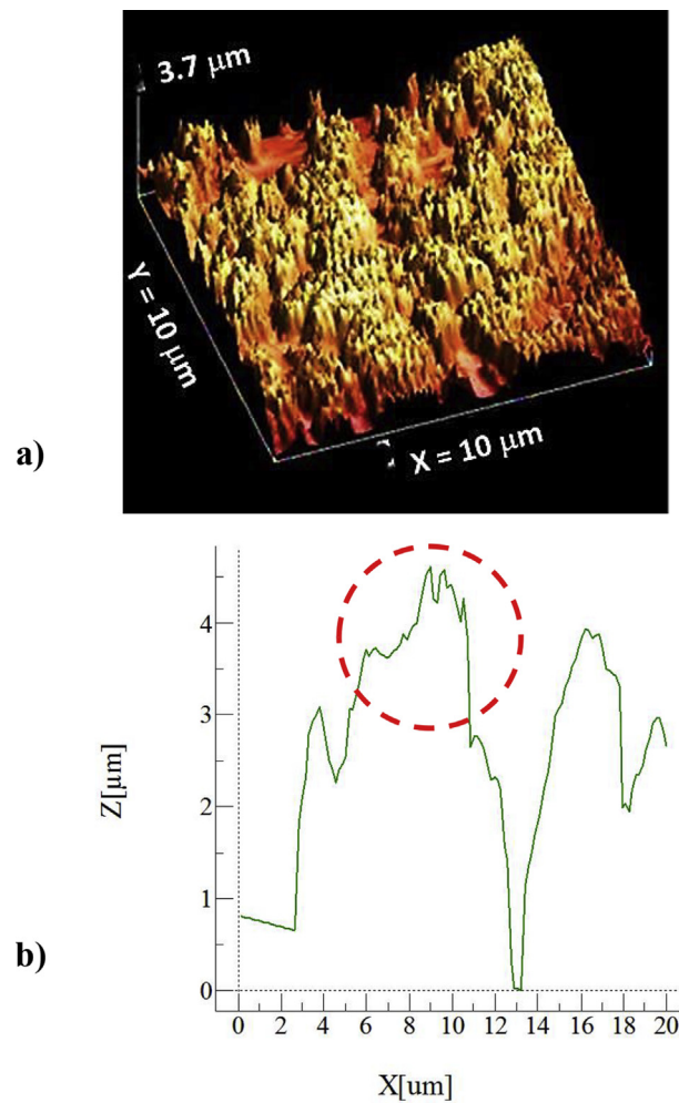
Fig. 2. AFM data for laser processed surface: a) 3D-image of laser processed surface, and b) line scan along the surface (the red dotted circle demonstrates the presence of nano-size structures).
