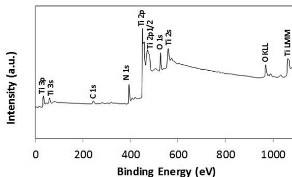
Fig. 4. XPS spectra for the laser treated surface.
