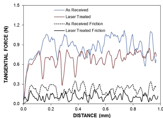
Fig. 11. Tangential and frictional forces along the scratch distance. Tangential force represents force needed removing dried solution from surface and frictional force is due to laser processed and untreated surfaces without dried solution presence.
