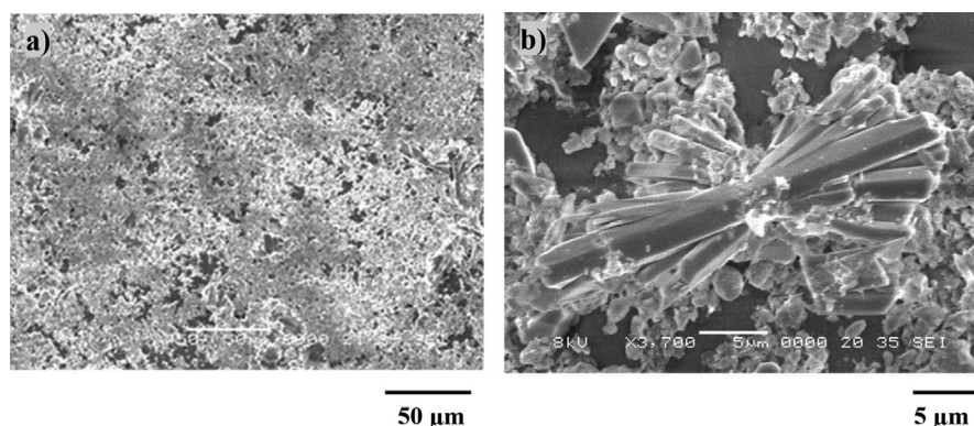
Fig. 10. SEM micrographs of dried solution: a) dried liquid solution covering laser processed surface, and b) crystallized dried solution on laser processed surface.
