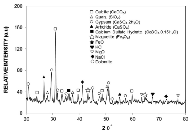
Fig. 9. X-ray diffractogram of dust.
