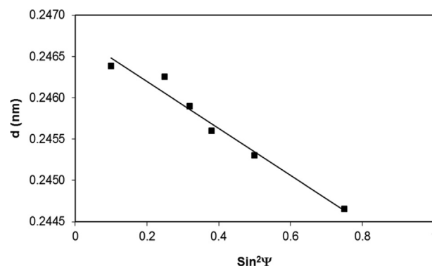
Fig. 6. Dependence of d-spacing with tilt angle.
