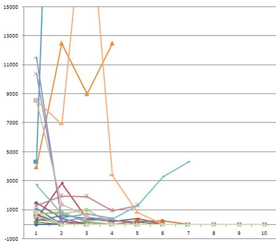
Figure 2. Dot plot showing trend of CMV viremia after leflunomide. Twenty episodes are included of 24 (3 patients had end-organ involvement without viremia and 1 patient discontinued all treatment).
