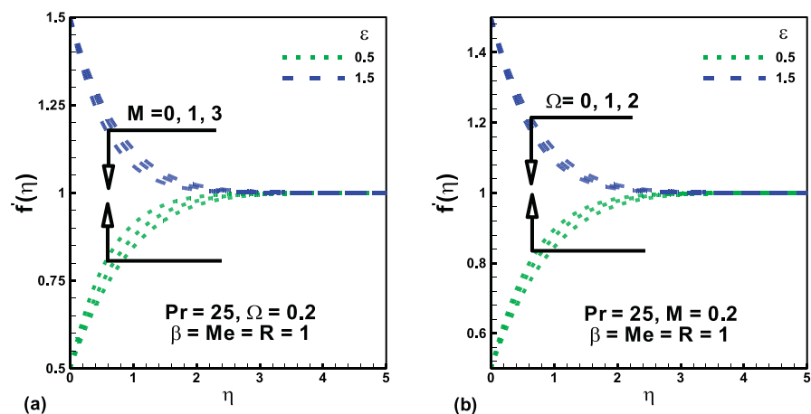
Fig. 2. (a) Effects of M and \varepsilon (b) Effects of \Omega , \varepsilon on the dimensionless velocity.
