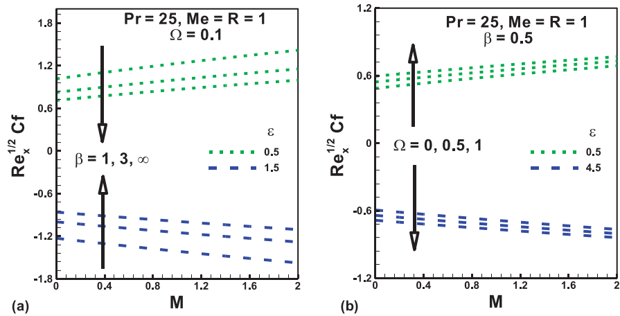
Fig. 8. (a) Effects of M , \beta and \epsilon (b) Effects of \Omega , M and \epsilon on skin friction coefficient.
