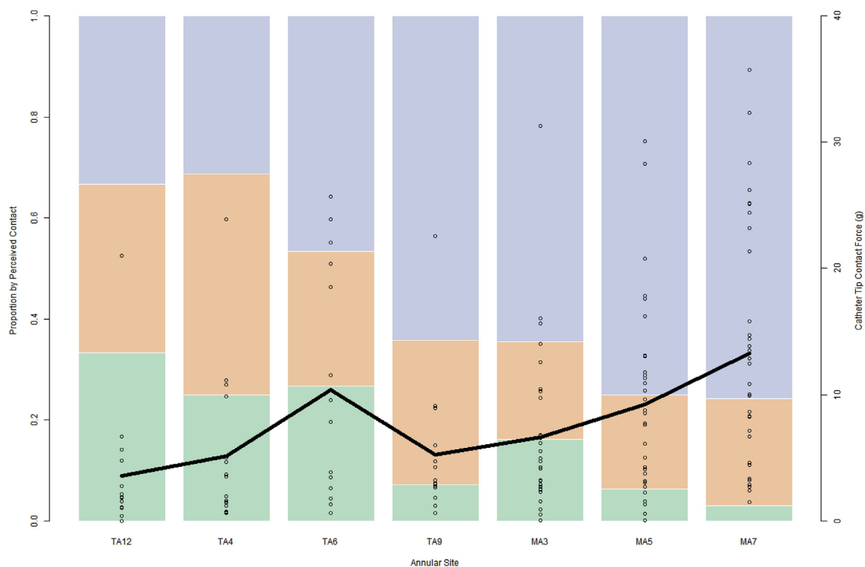
Fig. 2. Catheter to tissue contact by location. Stacked bars represent proportion of points collected at poor (bottom, green), moderate (middle, peach) and good (top, blue) perception of contact (left y axis). Dots represent scatter of measured contact force values obtained from each annulus position; line connects mean measured contact force obtained from each annulus position (right y axis). Annular site abbreviations as Fig. 1.
