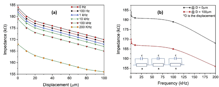
Fig. 3. (a) Dependences of resistance and impedance on the displacement for rubber-graphene layered composite. (b) The frequency vs impedance at different displacements, inset shows the simplified equivalent circuit of the elastic layered rubber-graphene composite samples.
