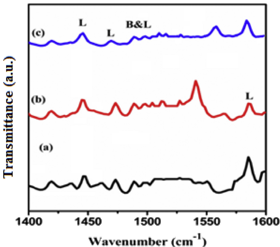
Fig. 5. Pyridine FT-IR patterns of (a) commercial \alpha -Fe 2 O 3 , (b) ARB clay, and (c) commercial silica catalysts.
