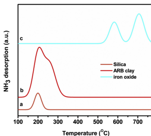
Fig. 4. \text{NH}_3 -TPD patterns of (a) commercial silica, (b) ARB clay, and (c) \alpha\text{-Fe}_2\text{O}_3 catalysts.
