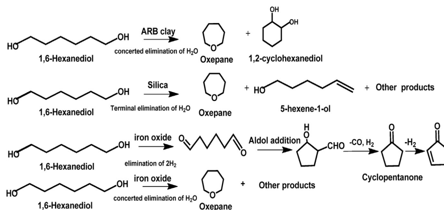
Fig. 9. 1,6-HDO dehydration procedure on ARB clay, commercial silica and \alpha -Fe 2 O 3 catalysts.
