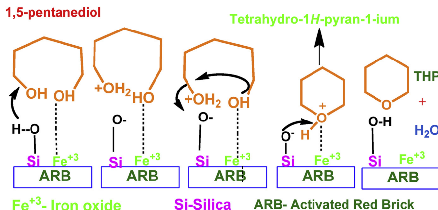
Fig. 14. A plausible reaction mechanism for 1,5-PDO dehydration on ARB catalyst.
