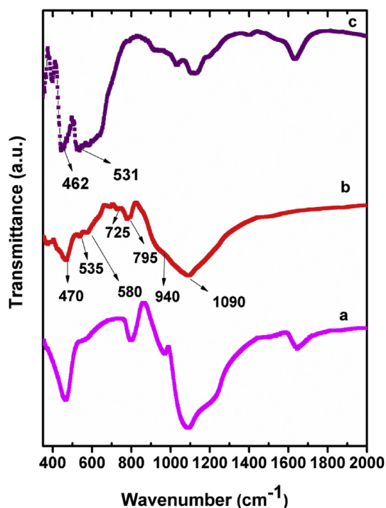
Fig. 2. FT-IR analysis of fresh (a) commercial silica, (b) ARB clay, (c) \alpha -Fe 2 O 3 catalysts.
