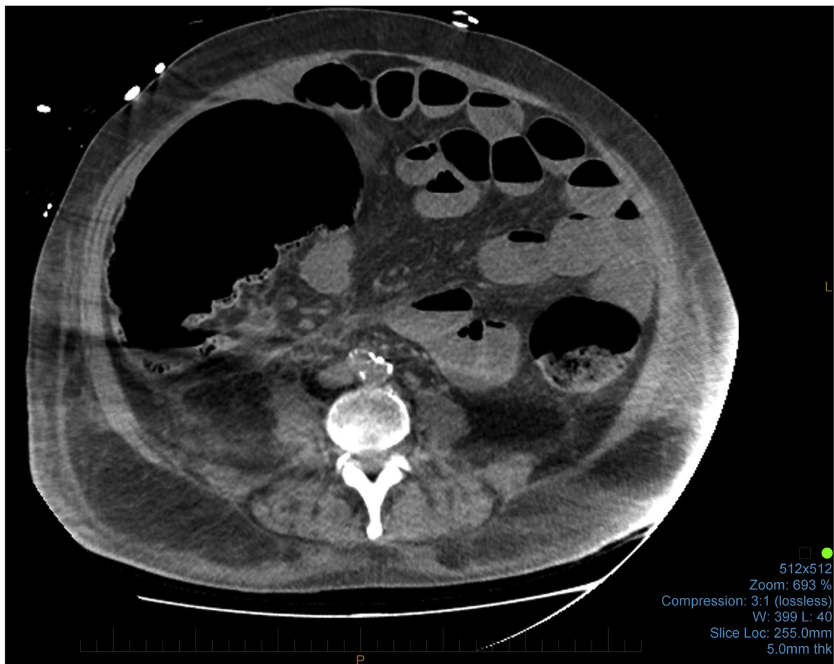
Fig. 1. CT demonstrating distension of caecum with ischaemia of caecal wall.
