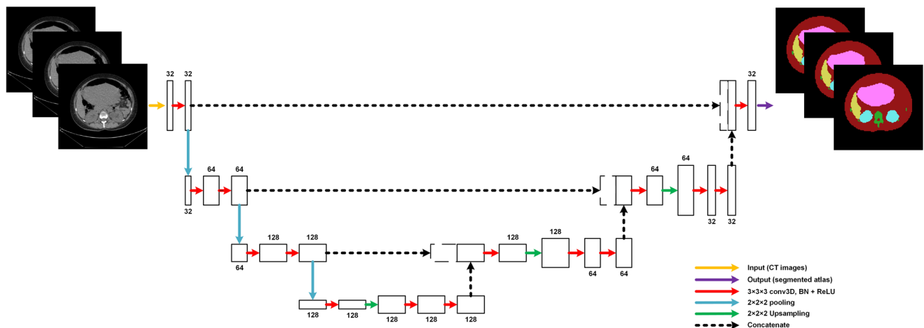
Fig. 1 Proposed convolutional neural network model used for automated segmentation of pregnant patients' CT images. BN refers to batch normalization whereas ReLU refers to rectified linear unit activation function
