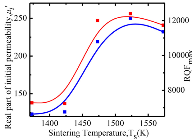
Fig. 8. Variation of \mu_i' at 1 MHz and RQF with different sintering temperatures of Li_{0.15}Ni_{0.3}Zn_{0.4}Fe_{2.15}O_4 .
