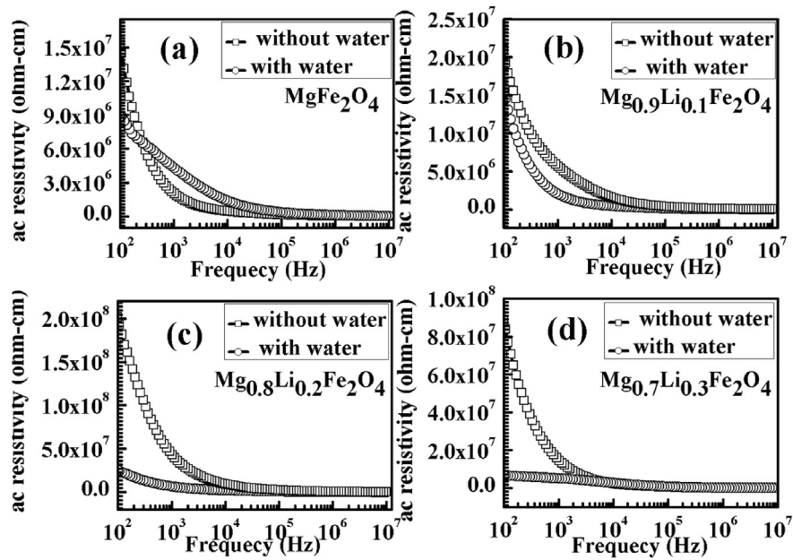
Fig. 8. Variation of resistivity of the \text{Mg}_{1-x}\text{Li}_x\text{Fe}_2\text{O}_4 samples, (a) x = 0.0 , (b) x = 0.1 , (c) x = 0.2 , (d) x = 0.3 , with and without water.
