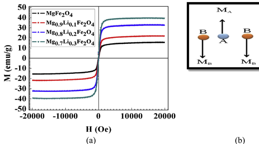
Fig. 5. (a) M-H loops of \text{Mg}_{1-x}\text{Li}_x\text{Fe}_2\text{O}_4 samples at room temperature and (b) Neel's collinear model to explain the magnetic behaviour in ferrites.
