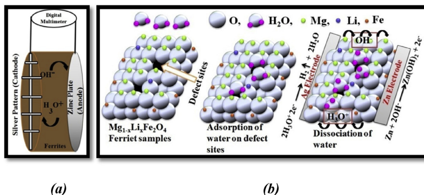
Fig. 6. (a) Schematic diagram of working of a hydroelectric cell and (b) representation of water adsorption and its dissociation on the surface of the \text{Mg}_{1-x}\text{Li}_x\text{Fe}_2\text{O}_4 samples.
