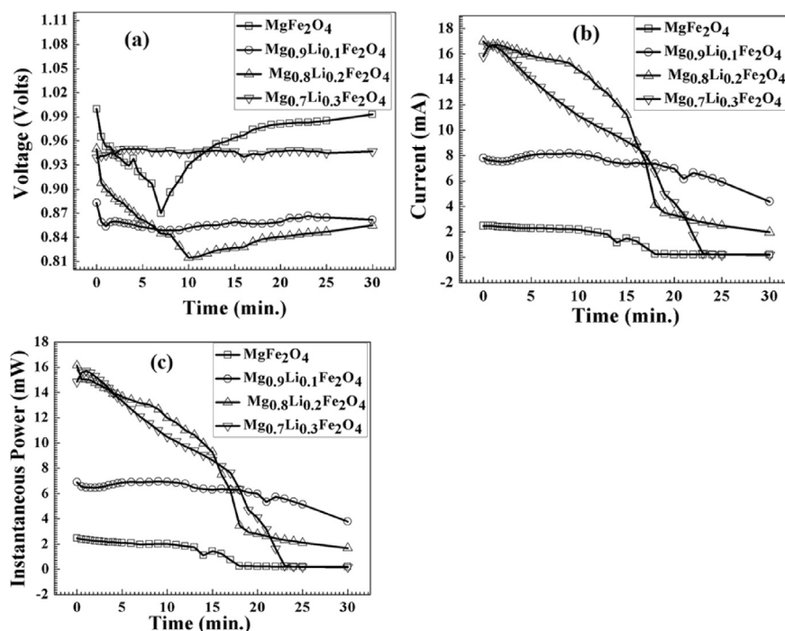
Fig. 7. (a) Voltage, (b) current and (c) power generated by hydroelectric cells of the \text{Mg}_{1-x}\text{Li}_x\text{Fe}_2\text{O}_4 samples.
