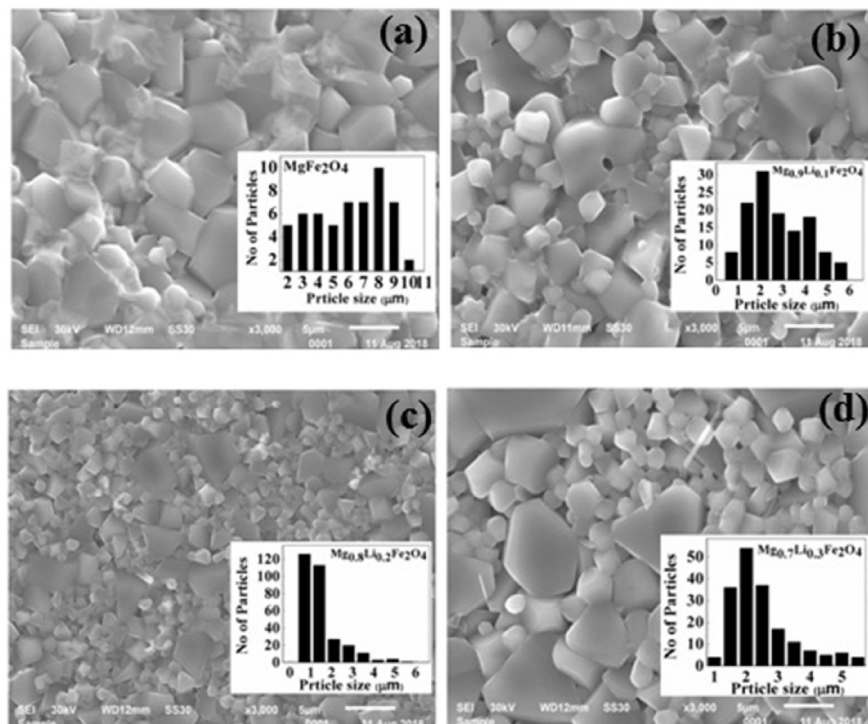
Fig. 4. SEM images of \text{Mg}_{1-x}\text{Li}_x\text{Fe}_2\text{O}_4 samples (a) x = 0.0 , (b) x = 0.1 , (c) x = 0.2 , (d) x = 0.3 and their grain size distribution (in-set).
