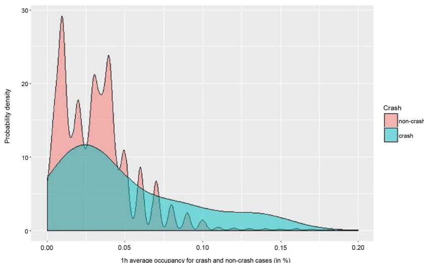
Fig. 3. Probability density of 1-hour average occupancy for crash and non-crash cases.
