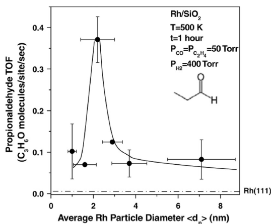
Fig. 29. Propionaldehyde TOF vs. average Rh particle size (nm). Reaction conditions: 50 Torr \text{C}_2\text{H}_4 ; 400 Torr \text{H}_2 at T = 500\text{ K} for 1 h. \pm\sigma_y error bars represent error of repeated reactivity measurements, \pm\sigma_x error bars represent the sigma of the Rh particle size distribution as determined from STM measurements (Adapted with permission from [34]. Copyright 2011, the National Academy of Sciences of the United States of America).
