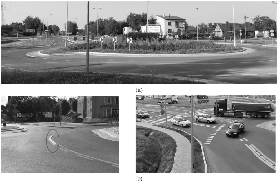
Fig. 2. Examples of research sites without lane dividers (a) and with different height of lane dividers (b).
