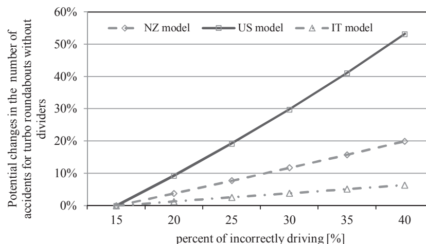
Fig. 11. The influence of incorrect passages on the change in the number of accidents for turbo-roundabouts.
