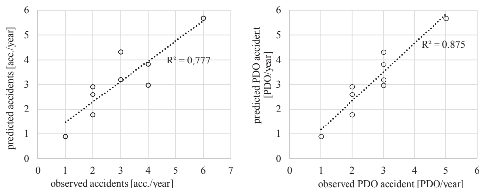
Fig. 5. Relationship between observed and predicted values for accidents and PDO accidents.
