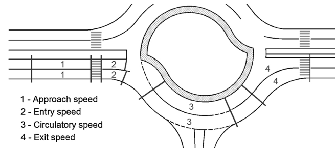
Fig. 3. Layout of measurement speed sections: 1 – approach ( S_{app} ), 2 – entry ( S_{en} ), 3 – circulatory roadway ( S_{cir} ), 4 – exit ( S_{ex} ).
