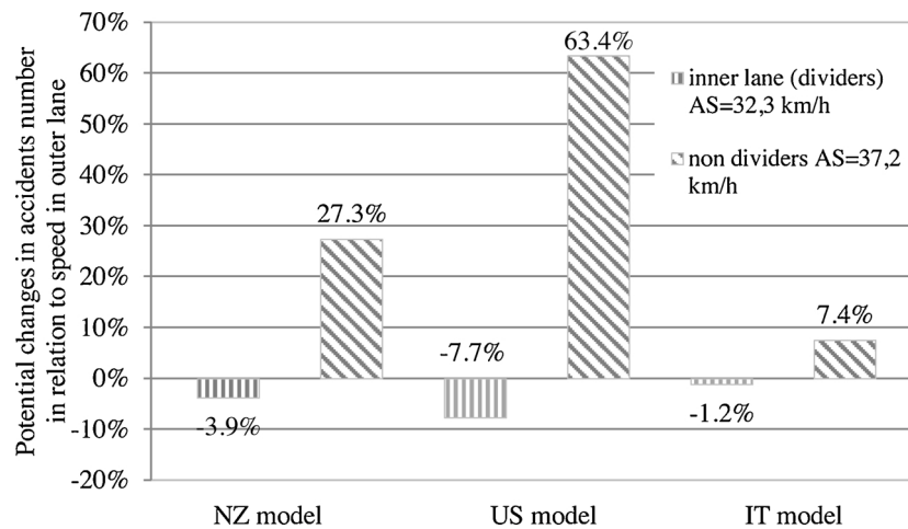
Fig. 10. The potential change in the number of accidents at turbo-roundabouts depending on the observed values of average speed.
