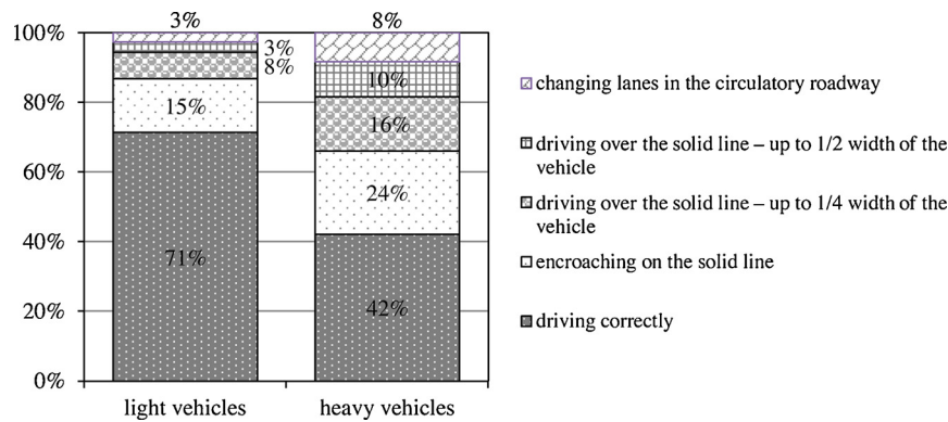
Fig. 7. Comparison of behaviours in turbo-roundabouts for light and heavy vehicles.
