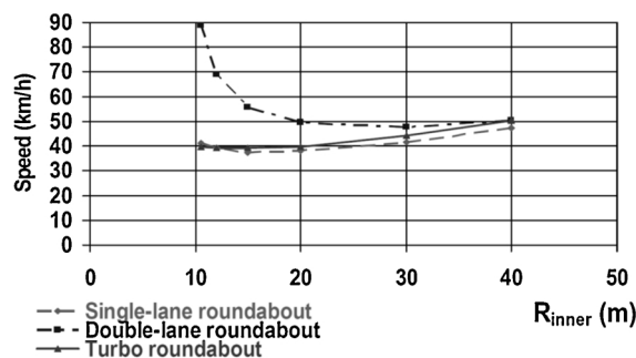
Fig. 1. The impact of the type of a circular intersection on the vehicle speed (Fortuijn, 2009).
