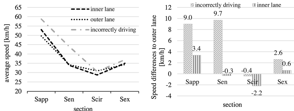
Fig. 8. Speed profile on the section of passing through the roundabout for correct and incorrect driving.
