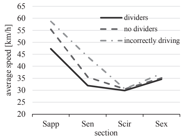
Fig. 9. Speed profile at the turbo roundabouts with and without lane dividers and incorrect driving.
