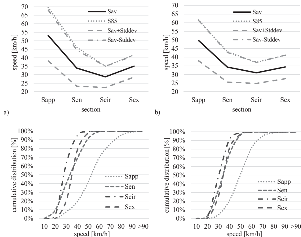
Fig. 6. Speed profile on the section of passing through the roundabout and speed distribution function for the inner lane (a) and the outer lane (b).
