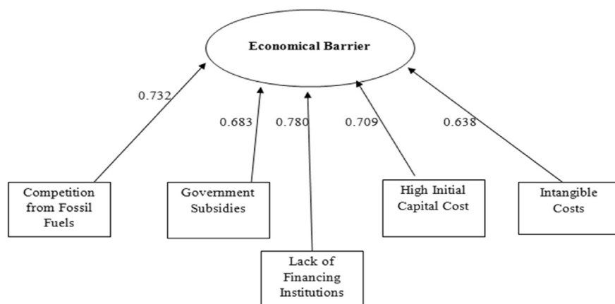
Fig. 4. Economic barriers with associated path coefficients.
