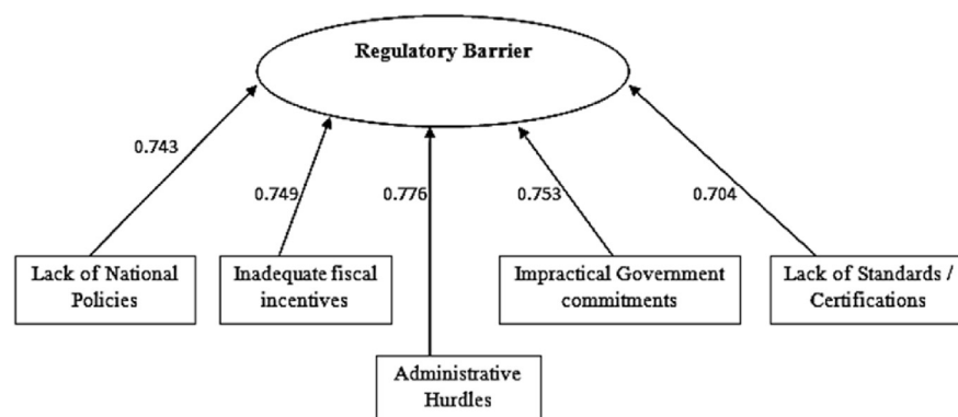
Fig. 6. Regulatory barriers with associated path coefficients.
