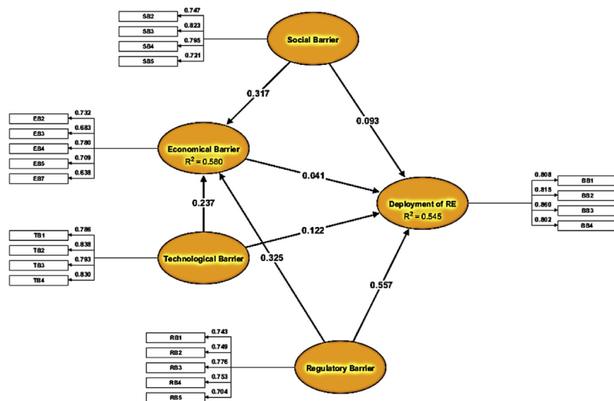
Fig. 2. Structural modelling through bootstrapping.
