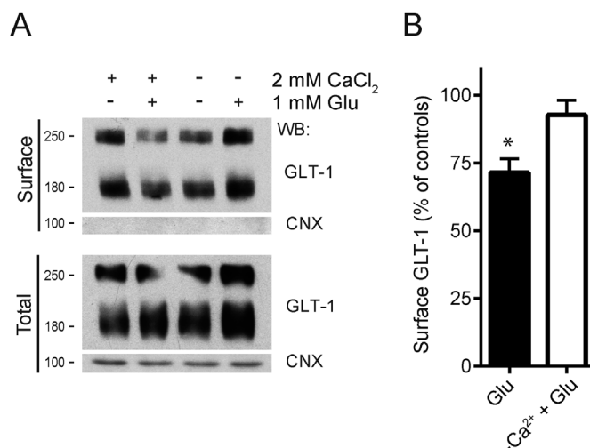
Fig. 1. Calcium dependent internalization of GLT-1 in primary mixed cultures. Rat brain mixed primary cultures were exposed to glutamate (1 mM) for 30 min in the presence or absence of calcium (2 mM \text{CaCl}_2 ). Cell surface proteins were labeled with NHS-Sulfo-biotin and after cell lysis, the biotinylated proteins (surface) were recovered with streptavidin-agarose beads and resolved by SDS-PAGE. Samples of the total cell lysate were run in parallel. GLT-1 expression was analyzed in Western blots and calnexin (CNX) immunodetection was used as a non-biotinylated protein control. The graph in B reflects the densitometric analysis of three independent immunoblots and it represents the mean \pm SEM, normalized to the total GLT-1 expression in each lane, and expressed as percentages of the respective controls (normalized intensities in the absence of glutamate): *, p < 0.05 by ANOVA with Bonferroni post-hoc test.
