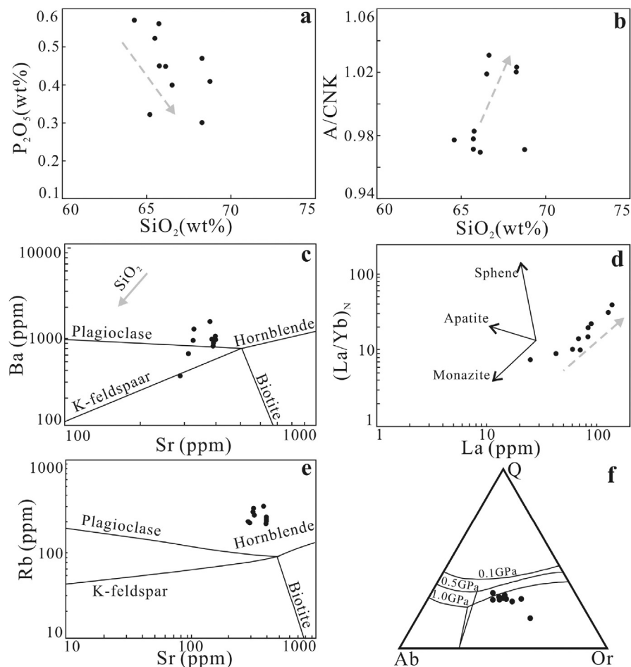
Fig. 5. Plots of (a) P_2O_5 vs. SiO_2 , (b) A/CNK vs. SiO_2 , (c) Ba vs. Sr, (d) (La/Yb)_N vs. La, and (e) Rb vs. Sr for the Alaer granite, illustrating that mineral fractionation is responsible for chemical compositions of the granite. Mineral fractionation vectors from Nash and Crecraft (1985), Bacon and Druitt (1988), Mahood and Hildreth (1983), Arth (1976). The average crustal composition from Weaver and Tarney (1984) is assumed to represent the initial melt composition. Grey dotted lines with arrows in (a), (b) and (d) show evolution trend of trace element concentrations. Plot of (f) CIPW-normative Q-Ab-Or diagram (Johannes and Holtz, 1996), showing the melt composition of the Alaer granite under high pressure. Q-quartz, Ab-albite, Or-orthosite.
