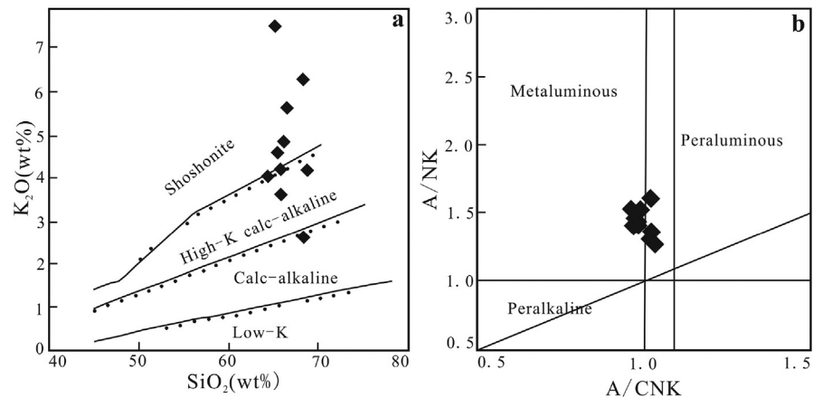
Fig. 3. Classification of the Alaer granite samples: (a) SiO 2 – K 2 O diagram (Rickwood, 1989). (b) A/CNK – A/NK diagram (Maniar and Piccoli, 1989). (A/NK = molar ratio of Al 2 O 3 /[K 2 O + Na 2 O]; A/CNK = molar ratio of Al 2 O 3 /[CaO + K 2 O + Na 2 O]).
