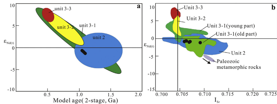
Fig. 6. \epsilon_{\text{Nd}(t)} vs. T_{\text{DM}} diagram (a) and \epsilon_{\text{Nd}(t)} vs. I_{\text{Sr}} ( (^{87}\text{Sr}/^{86}\text{Sr})_I ) diagram (b) for the Alaer granite. The coloured areas represent the granitoids and Paleozoic metamorphic rocks from the Chinese Altay (Wang et al., 2009, 2014). T_{\text{DM}} is Nd model age. Unit 2, 3-1, 3-2 and 3-3 correspond to those of Fig. 1a. These two figures illustrate the Alaer granite could have been produced by melting of sources which were formed ca. 1.6–1.0 Ga ago and an initial melt was generated by partial melting of older continental basement or mixed with mantle-derived magma.
