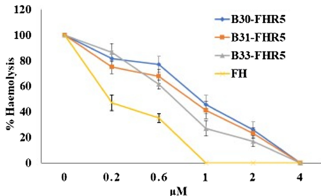
Fig. 4. Inhibition of haemolysis by FHR5. The volume 20 µL of FH family depleted serum capable of giving 50% haemolysis was mixed with DGV-B-Mg-EGTA, sheep erythrocytes and varying concentrations of FHR5 or FH (0.2–4 µM). Haemolysis observed is displayed as percentage of the lysis of FH family depleted serum without additions. The experiments were carried out in triplicates. Error bars represent standard deviation.
