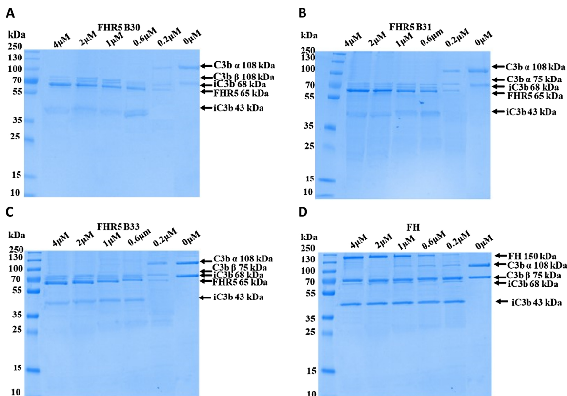
Fig. 5. GBM-FHR5 has factor I-cofactor activity. Varying doses between 0.2–4 \mu M of GBM-FHR5 were incubated with 3 \mu g of C3b, 45 ng of Factor I in 10 mM sodium phosphate (pH 6.0) for 10 min at 37 °C. Reactions without GBM-FHR5 or FH and were included as controls. Cleavage of C3b was analysed by SDS-PAGE using Coomassie blue staining.
