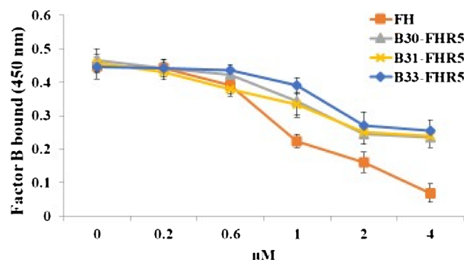
Fig. 6. FHR5 promotes decay acceleration activity on C3 convertase. C3 convertase was generated in microtiter plates with 250 ng of C3b, 400 ng of factor B, 25 ng of factor D, 2 mM nickel chloride, 25 mM NaCl and 4% BSA for 2 h at 37 °C. Varying concentrations of FHR5 (0.2–4 \mu M) were added and incubated for 30 min at 37 °C. FH and samples without FH and FHR5 were included as controls. Intact C3 convertase was detected by goat anti-human factor B and rabbit anti-goat IgG-HRP antibody. The colour was developed with o-Phenylenediamine. The experiment was repeated in triplicates. Error bars represent standard deviation.
