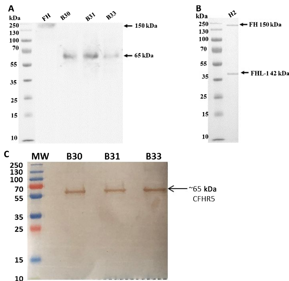
Fig. 1. Western blot analysis of serum free primary GBM supernatant. 0.2 \times 10^6 (A) B30, B31, B33 (B) and H2 cells (control). Cells were grown for 48 h at 37 °C with 5% v/v \text{CO}_2 in the absence of fetal calf serum. The culture supernatant was collected and an SDS-PAGE was run (reduced samples). FH was included as a control. The samples were transferred onto nitrocellulose membrane and probed with polyclonal rabbit polyclonal anti-FH (10 \mu\text{g} IgG/mL) and anti-rabbit IgG-HRP (5 \mu\text{g} /mL) antibodies for 1 h. The detected protein band was visualised using 3,3'-diaminobenzidine. (c) The purified proteins were also probed with goat anti-FHR5 polyclonal antibodies (1:1000; R&D; cat. no. AF3845-SP).
