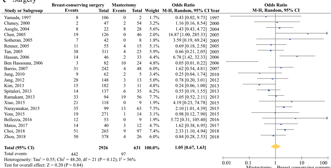
FIG. 2 a Forest plot showing the pooled odds ratios (ORs) of local recurrence (LR) by age. All studies used 40 years as the cutoff except for Wei et al. 62 (35 years) and Zhou et al. 18 (38 years). b Forest plot showing the pooled ORs of LR by tumor size (> 5 vs. ≤ 5 cm) except for Kim et al. 15 (4 cm). c Forest plot showing the pooled ORs of LR by surgery type (breast-conserving surgery vs. mastectomy). d Forest plot showing the pooled ORs of LR by surgical margin (positive vs. negative). The surgical margin width in each study was marked in the footnote. The study without a footnote
