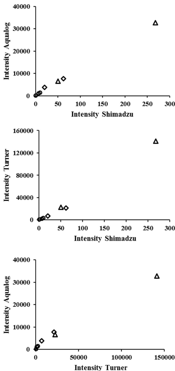
Fig. 2. Comparison of fluorescence intensity of samples using three different fluorometers. Samples were extracted in dichloromethane. WAF ( \diamond ), CEWAF ( \Delta ), and Oil Standard ( \circ ). See Table 2 for statistical results.
