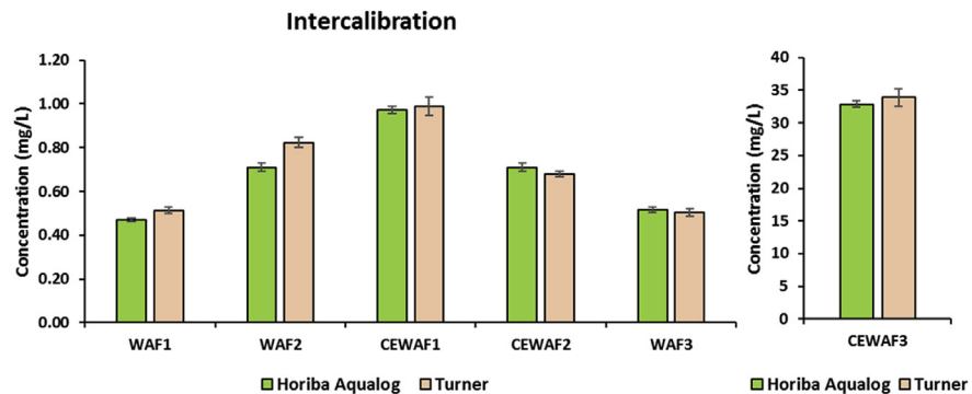
Fig. 4. Equivalent Oil Equivalent (EOE) results for intercalibration samples of exercise 2. Results are given as means \pm standard deviation. See Tables 3 and 4 for error values. Note the change of scale between the two panels.
