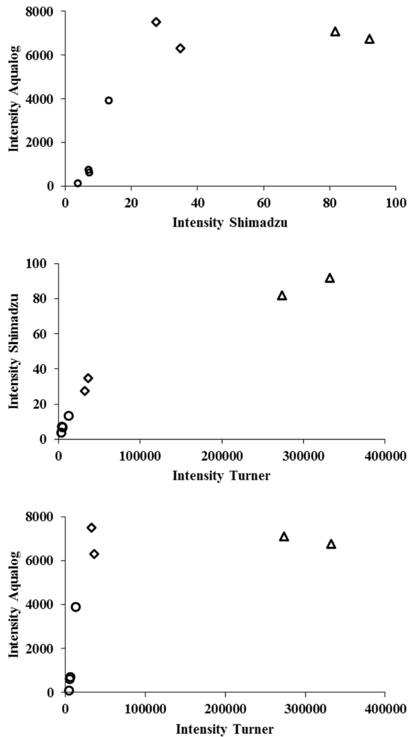
Fig. 1. Comparisons of fluorescence of samples from intercalibration 1 without extraction, expressed as relative fluorescence units using three different fluorimeters. WAF (◇), CEWAF (Δ), and Oil Standard (○). See Table 1 for statistical results.
