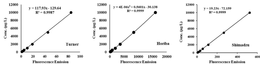
Fig. 3. Calibration curve of surrogate Macondo oil in dichloromethane determined in the Horiba Aqualog, Turner Trilogy (module 7200-063), and Shimadzu fluorometer.
