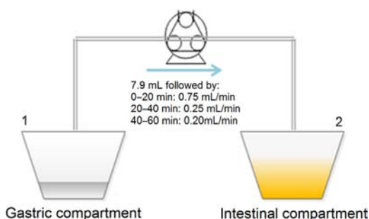
Figure 1 Schematic representation of the rat in vitro lipolysis model. Gastric (1) and intestinal compartments (2) are connected by a peristaltic pump. Initially, 7.9 mL of the gastric content were transferred manually followed by the flows described above.
