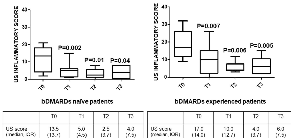
Fig. 2 Box and whiskers plot (median, quartiles, range) of US inflammatory score of naïve or bDMARD-experienced PsA patients at baseline (T0) and after 6 (T1), 12 (T2), 24 weeks (T3) of treatment with apremilast. P values were referred to the comparison with baseline
