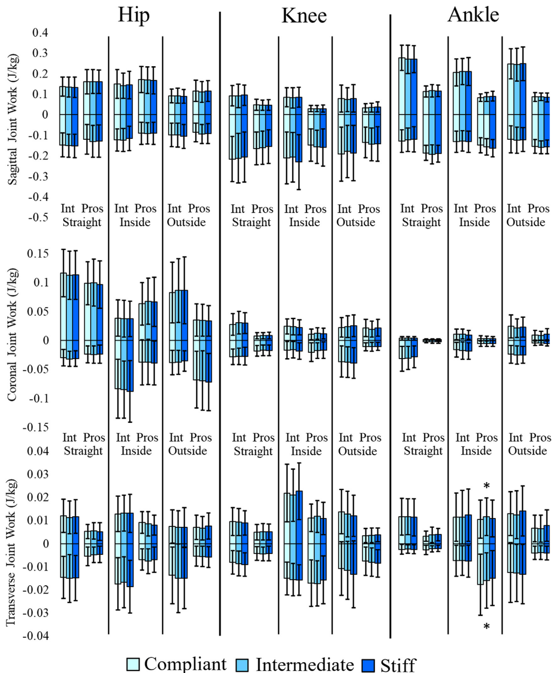
Fig. A2. Joint work mean ( \pm 1 standard deviation) for each stiffness setting across walking speeds during the stance phase for the Intact (Int) and Prosthetic (Pros) limbs. Activities defined as straight-line walking (Straight), limb on the inside of the turn (Inside) and limb on the outside of the turn (Outside). Stiffness levels defined as: compliant 0.25 Nm/°, intermediate: 0.75 Nm/° and stiff: 1.25 Nm/°. Means were normalized by participant mass. Significant difference ( p < 0.05 ) indicated with *.
