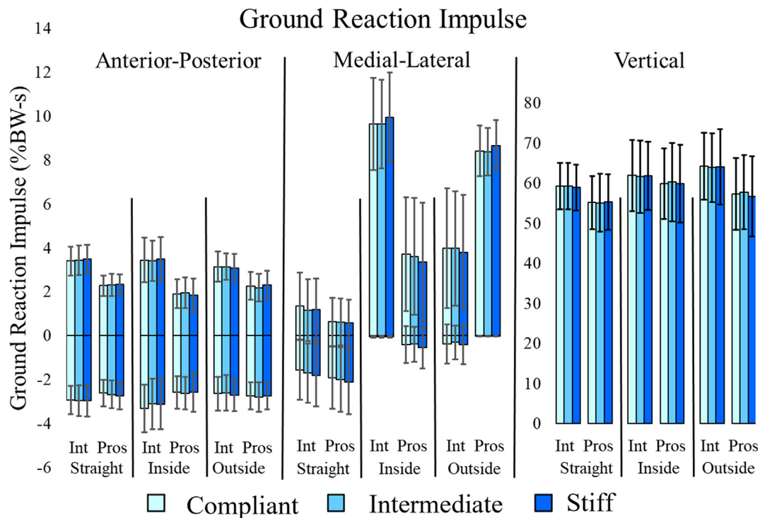
Fig. A1. Ground reaction impulse mean ( \pm 1 standard deviation) for each stiffness setting across walking speeds during the stance phase for the Intact (Int) and Prosthetic (Pros) limbs. Activities defined as straight-line walking (Straight), limb on the inside of the turn (Inside) and limb on the outside of the turn (Outside). Stiffness levels defined as: compliant 0.25 Nm/°, intermediate: 0.75 Nm/° and stiff: 1.25 Nm/°. Means were normalized by participant mass.
