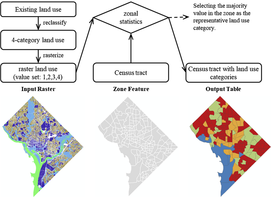
Fig. 5. The Process of Assigning Land Use Categories to Census Tracts.
