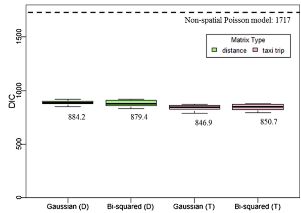
Fig. 7. DIC Evaluation Results with 15 Runs of Sampling Process.
