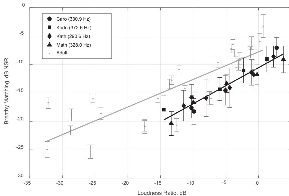
FIGURE 3. Matching NSR by loudness ratio in dB. The mean \pm SE are given, averaged over all listeners. Black symbols are for pediatric voices, with symbol type separating the four different talkers. Gray symbols correspond to adult voices from Shrivastav et al. 52 Lines with the same shading scheme represent linear regression. In both cases, goodness of fit was high (pediatric voices: r^2 = 0.93 ; adult voices: r^2 = 0.72 ).
