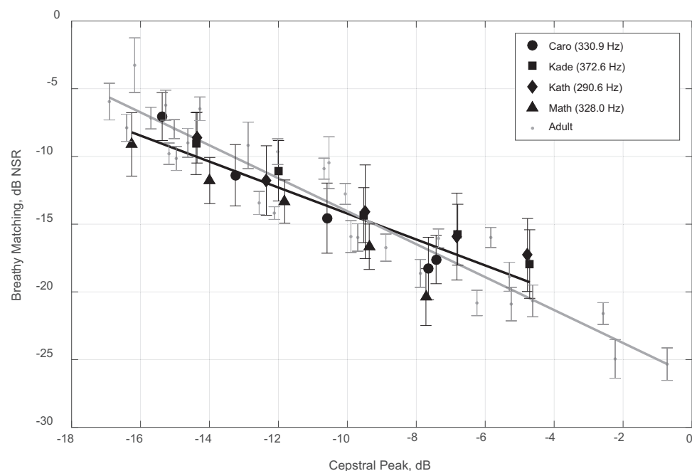
FIGURE 5. Matching NSR by cepstral peak in dB. The mean \pm SE are given, averaged over all listeners. Black symbols are for pediatric voices, with symbol type separating the four different talkers. Gray symbols correspond to adult voices from Shrivastav et al. 52 Lines with the same shading scheme represent linear regression. In both cases, goodness of fit was high (pediatric voices: r^2 = 0.82 ; adult voices: r^2 = 0.91 ).
