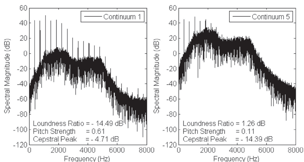
FIGURE 1. Fourier spectra of AH-OQ for two synthetic talkers. Both talkers are based on the same natural voice and represent the two end points of the breathy continuum (continuum positions 1 and 5), where position 1 represents a voice with a low degree of breathiness and position 5 represents a voice with high degree of breathiness. Values in the inset of each panel highlight the acoustic indices described in the text.
