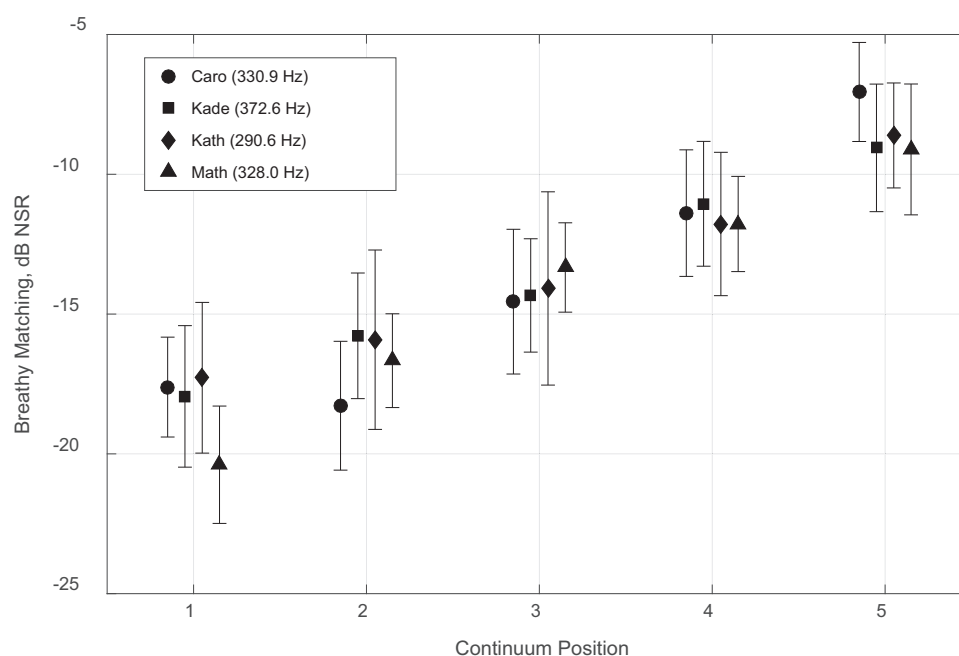
FIGURE 2. Matching NSR by continuum position. The mean \pm SE are given, averaged over all listeners.
