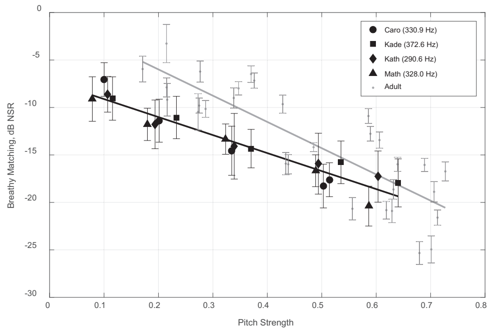
FIGURE 4. Matching NSR by pitch strength. The mean \pm SE are given, averaged over all listeners. Black symbols are for pediatric voices, with symbol type separating the four different talkers. Gray symbols correspond to adult voices from Shrivastav et al. 52 Lines with the same shading scheme represent linear regression. In both cases, goodness of fit was high (pediatric voices: r^2 = 0.91 ; adult voices: r^2 = 0.71 ).
