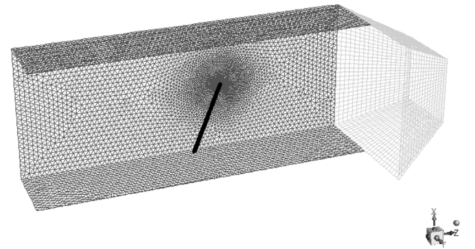
Fig. 7. Mesh for rigorous simulation. Showing only one side of the channel wall.
