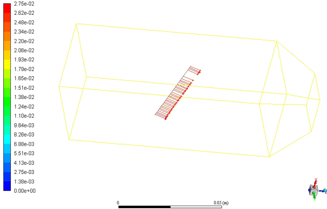
Fig. 10. Force per chord length calculated by ALM, [N/m]. Peak systole (velocity U = 0.2 m/s).
