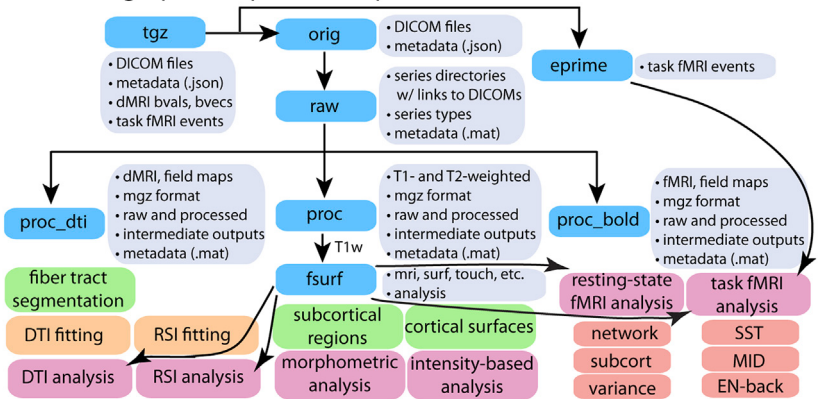
Fig. 1. Processing pipeline diagrams. A. Modality-specific processing steps for bias field, distortion, and/or motion correction. B. Processing pipeline input and outputs.
