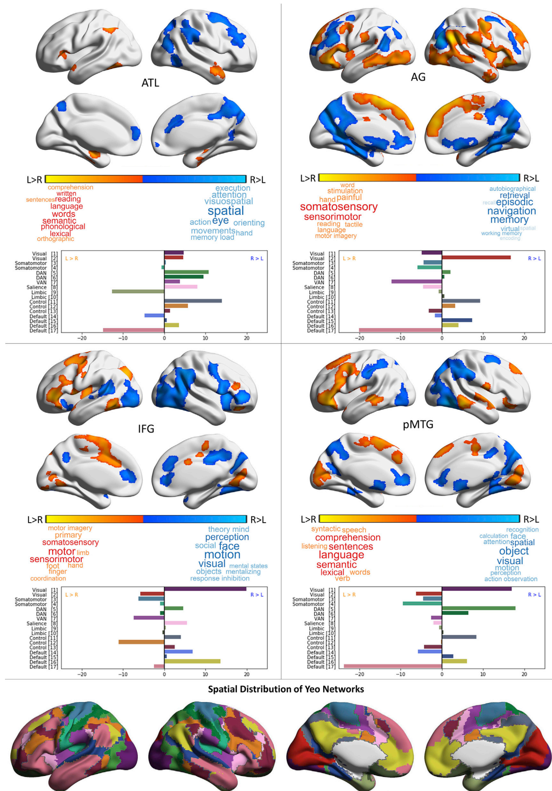
Fig. 5. Intrinsic connectivity group maps showing differences in the network topography (shape/magnitude) of connectivity patterns for left and right hemisphere seeds. The connectivity patterns for right hemisphere seeds were ‘flipped’ into left hemisphere space, and the maps therefore characterise differences in the shapes and magnitudes of largely symmetrical patterns of connectivity for the two hemispheres ( z = 3.1 , p < .05 ); these patterns are depicted in Fig. S3. The results of cognitive decoding using Neurosynth (Yarkoni et al., 2011) are shown in the word clouds below the colour bars. The charts for each seed show a comparison of these spatial maps with the Yeo et al. (2011) 17 networks (depicted in the bottom row, colour-coded to match the bar plots). Each chart plots the difference in overlap for each network from Yeo et al., comparing the LH > RH and RH > LH connectivity maps. A left-facing bar corresponds to more extensive overlap with the left-lateralised connectivity map, while a right-facing bar corresponds to more extensive overlap with the right-lateralised connectivity map. The network names and colour codes are taken from Shinn et al. (2015).
