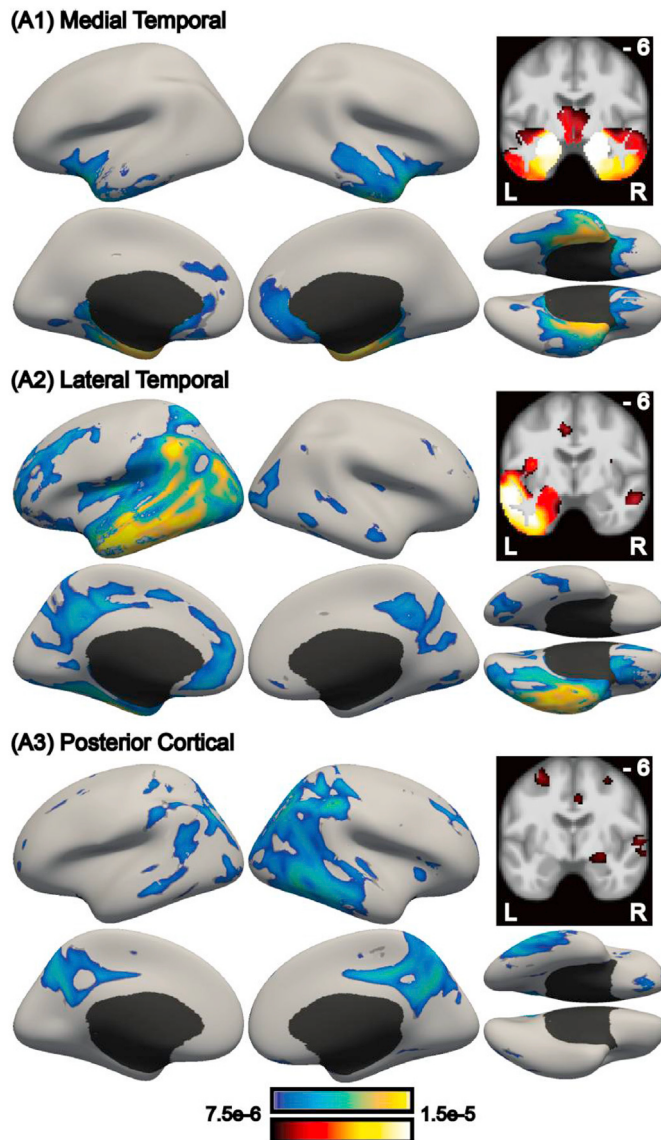
Fig. 3. Probabilistic atrophy maps of three latent factors in ADNI-GO/2. Brighter color indicates higher probability of atrophy at that voxel for a particular factor (i.e., \text{Pr}(\text{Voxel} \mid \text{Factor}) ). Each of the three factors was associated with a distinct pattern of brain atrophy. Coronal slices are found in Fig. S2.
