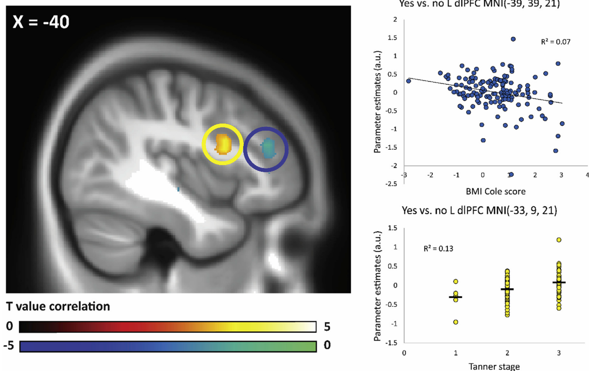
Fig. 2. Correlation of Tanner stage and BMI Cole score with modulation of choice activation by yes vs. no independent of condition. Blue circle denotes negative correlation with BMI Cole score and yellow circle denotes positive correlation with Tanner stage. Peaks listed are significant at the p < 0.05 level based cluster level corrections across the whole brain (individual voxel threshold = p < 0.001 , cluster extent threshold > 57 voxels, 3 \times 3 \times 3 mm voxels) and within an a priori set of regions of interest (individual voxel threshold p < 0.001 , cluster extent > 28 voxels, 3 \times 3 \times 3 mm voxels).
