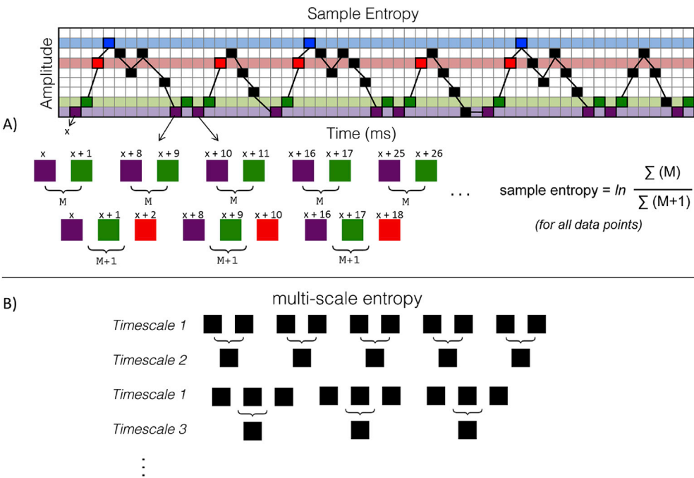
Fig. 2. Reprinted from Grundy et al. (2017). Bilinguals have more complex EEG brain signals in occipital regions than monolinguals. NeuroImage , 159, 280–288, with permission from Elsevier. Calculation of sample entropy and multiscale entropy using EEG brain signal. Panel A shows how to calculate sample entropy at each timescale. A criterion length m (2 in the present study) defines a number of consecutive data points in the EEG signal. For length m = 2 (starting with x and x+1 ), sum the number of times that two consecutive data points occur within a pre-specified amplitude range ( r = 0.5 in the present study) across time in the EEG waveform. Next, sum the number of times that three ( m + 1 ) consecutive data points (starting with x , x+1 , and x+2 ) occur within the amplitude range across time in the EEG waveform. This procedure is repeated for each data point in the time series (i.e., starting at x+1 , then starting at x+2 , then starting at x+3 , etc.) and all two-component matches and all three-component matches in the entire data series are summed together. Sample entropy is the natural logarithm of the ratio of two-component to three-component matches. Panel B represents downsampling of the original EEG data so that multiple fine to coarse timescales are created. This is done by averaging consecutive data points to create a new data point that corresponds to a coarser scale. This is done n times (in our study n = 20 ) and sample entropy is re-calculated at each timescale. This creates a series of fine to coarse grained entropy scales. This figure was inspired by Fig. 1 from Heisz et al. (2012).
