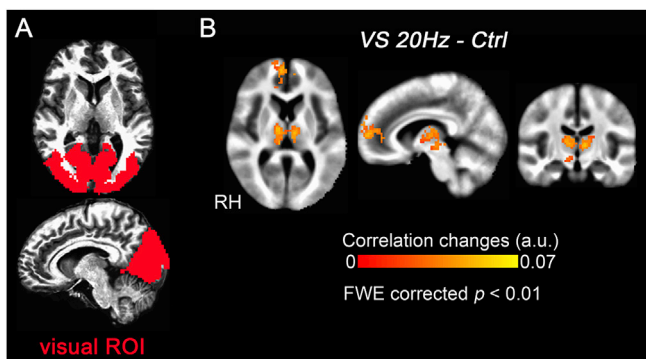
Fig. 7. Group-level correlation changes with the visual ROI ( N = 20 ). (A) The activated visual occipital region that was defined as the visual ROI. (B) Compared with the control condition, visual stimulation at 20 Hz (VS 20 Hz) significantly increased the correlation between the medial thalamus and the visual ROI. The medial frontal gyrus also shows significantly increased correlation with visual ROI. RH marks the side of right hemisphere.
