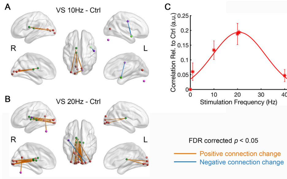
Fig. 6. Results of network statistical analysis and the tuning curve of thalamo-visual correlation ( N = 20 ). Compared to control, visual stimulation at (A) 10 Hz and (B) 20 Hz significantly enhanced the connectivity between thalamus and visual cortex. The purple nodes outside of the brain are cerebellar region. (C) Mean correlation between thalamus and visual cortex (arbitrary unit, a. u.) was plotted as a function of stimulation frequency. The asterisks indicate the measured correlations relative to control and the curves are the Gaussian functions that best fit the data. The star indicates the peak frequency of the fitted curve. The error bars indicate \pm SEM across subjects. R and L mark the side of left/right hemisphere.
