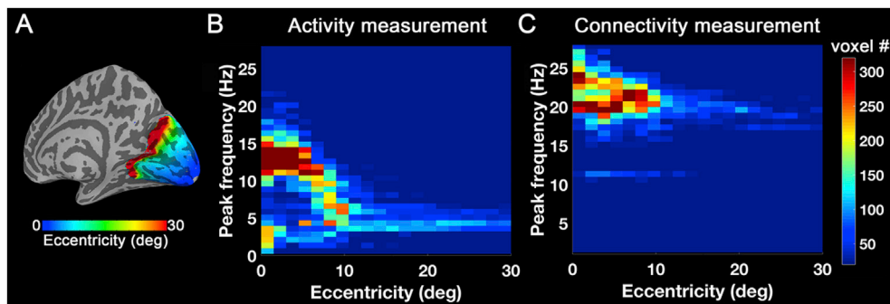
Figure 10. 2D-histogram across eccentricity and peak frequency. (A) Eccentricity template from Benson et al. (2014). (B) Number of voxels as a function of eccentricity and peak frequency for the group-level preferred frequency map of BOLD signal changes. (C) Number of voxels as a function of eccentricity and peak frequency for the group-level preferred frequency map of correlation changes.
