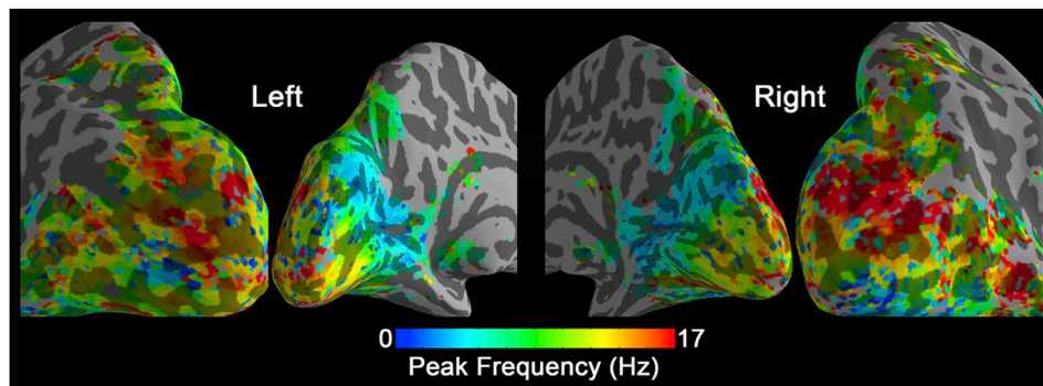
Fig. 4. Peak frequency map of group-level BOLD signal changes ( N = 17 ). In each voxel, the peak frequency was generated by fitting the BOLD signal changes vs. temporal frequencies.
