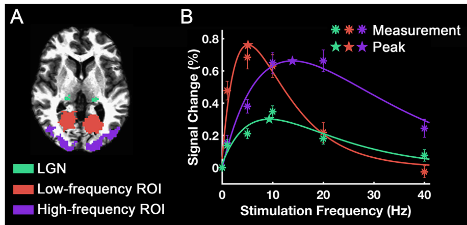
Fig. 3. Frequency tuning curves of different ROIs. (A) ROI areas. (B) ROI-mean signal change was plotted as a function of stimulation frequency. The asterisks indicate the measured signal changes. The curves are the difference of exponential functions that best fit the data. The stars indicate the peak frequencies of each curve. The error bars indicate \pm the standard error of the mean (SEM) across subjects ( N = 17 ).
