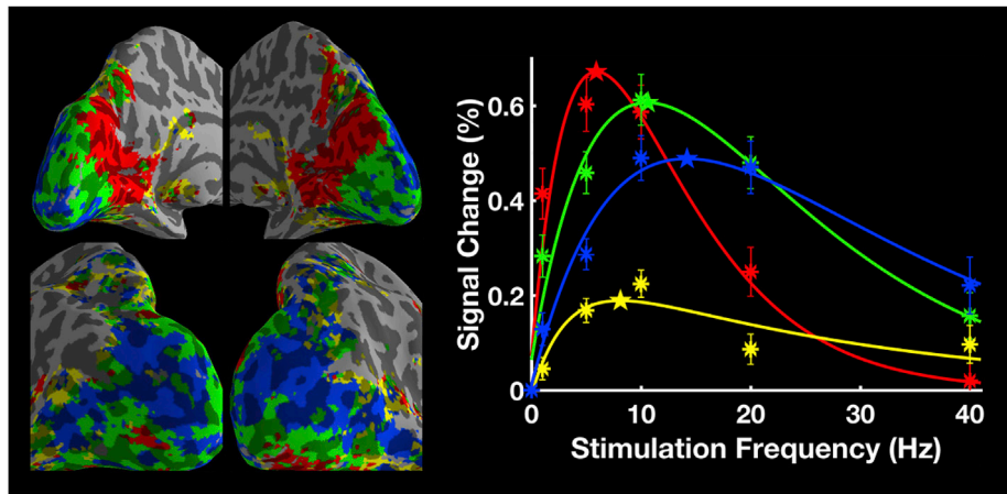
Figure 5. k -means parcellation ( k = 4 ) based on group-level frequency-dependent BOLD signal changes ( N = 17 ). The mean BOLD signal changes for each cluster are plotted as a function of stimulation frequency. The asterisks indicate the measured signal changes and the stars mark the peak frequency of each curve. The error bars indicate \pm SEM across all subjects.
