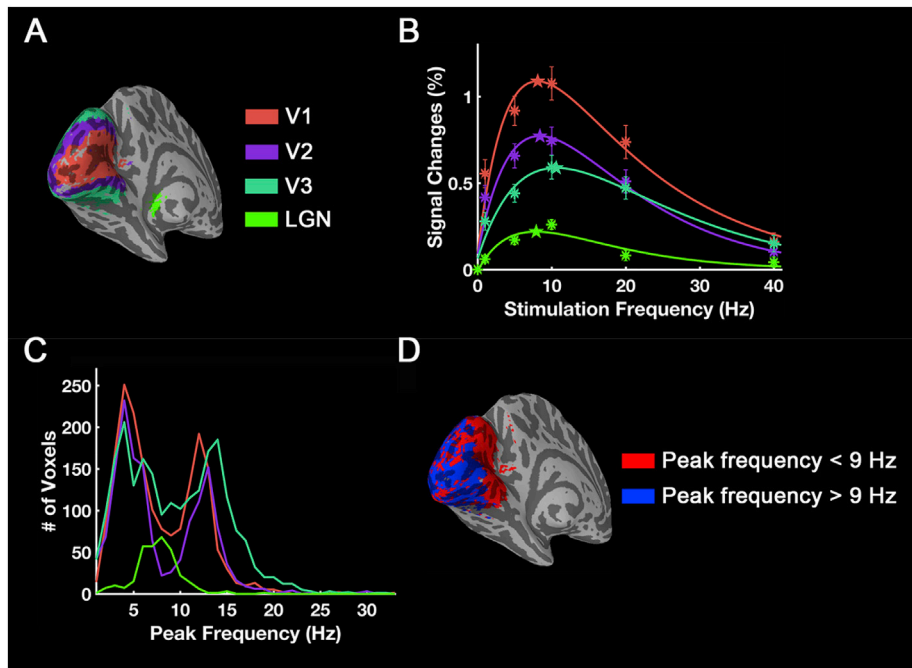
Fig. 11. Frequency tuning curves and histograms across visual areas for group-level activation. (A) V1/2/3 were defined by taking the intersection of the visual areas template from Benson et al. (2014) and preferred frequency mapping regions. Using measured BOLD magnitude changes, frequency tuning curves for different visual areas are shown in (B), and the histogram (C) shows how many voxels have a specific peak frequency. The color of the curves and points correspond to different visual areas. Asterisks are the measured mean value from each visual area and the stars mark the peak frequency of each fitted curve. The error bars indicate \pm SEM across subjects ( N = 17 ). (D) Distribution of areas with preferred frequency < 9 Hz and > 9 Hz.
