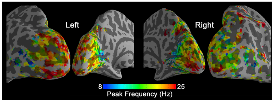
Fig. 8. Preferred frequency map of group-level correlation changes ( N = 20 ). In each voxel, the peak frequency was generated by fitting the frequency-dependent correlations with medial thalamus.
