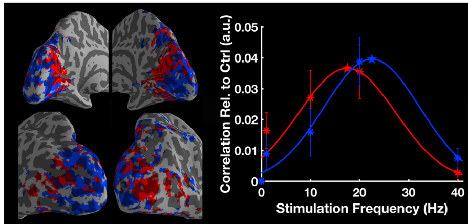
Figure 9. k -means parcellation based on frequency-dependent correlation changes to the thalamus at the group level ( N = 20 ). k = 2 was used and the mean correlation for each cluster was plotted as a function of stimulation frequency. The asterisks indicate the measured correlations relative to control, and the stars mark the peak frequency of each fitted curve. The error bars indicate \pm SEM across subjects.
