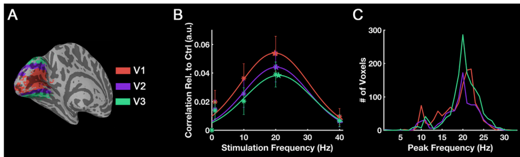
Fig. 12. Frequency tuning curves and histograms across visual areas for group-level correlation. Based on the thalamo-visual correlation, frequency tuning curves for different visual areas are shown in (B), and the histogram (C) shows how many voxels have a specific peak frequency. The color of the curves and points correspond to different visual areas. Asterisks are the measured mean value from each visual area and the stars mark the peak frequency of each fitted curve. The error bars indicate \pm SEM across subjects ( N = 20 ).
