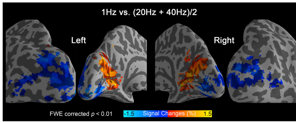
Fig. 2. Group activation differences for low (1 Hz) vs. high (20 Hz and 40 Hz) frequency stimulation (17 subjects).
