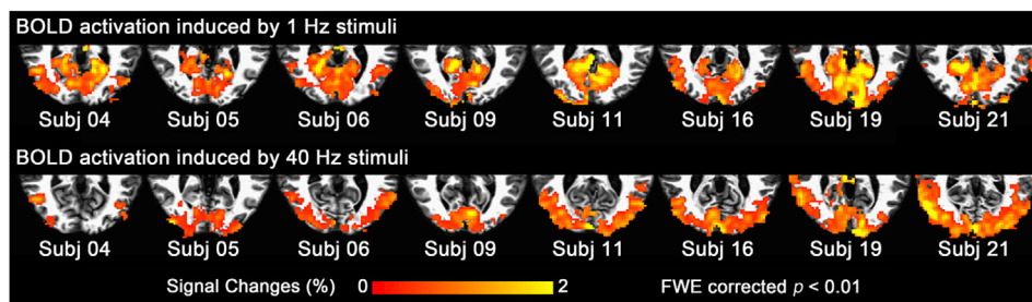
Fig. 1. Activation maps from 8 representative subjects. The upper row shows that 1 Hz stimuli caused significant activation across most of the calcarine sulcus, while the bottom row shows that 40 Hz stimuli resulted in relatively more significant activation in lateral occipital cortex.
