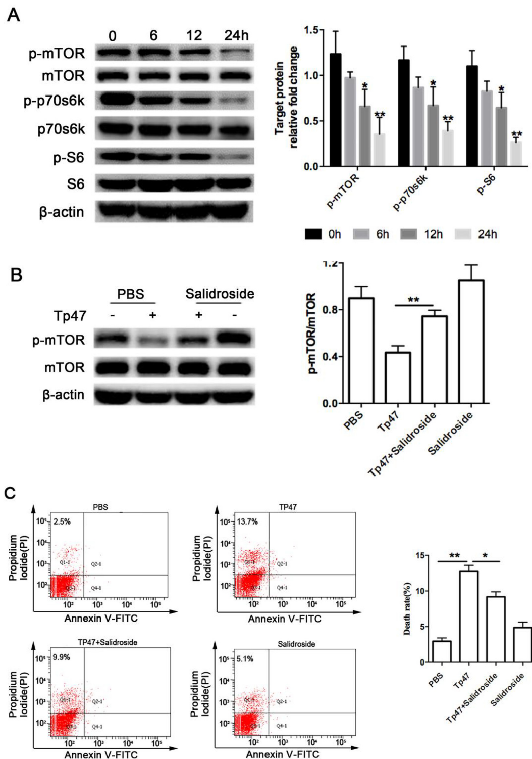
Fig. 4. Analysis of p-mTOR, p-p70s6k and pS6 expression levels in HMO6 cells.
