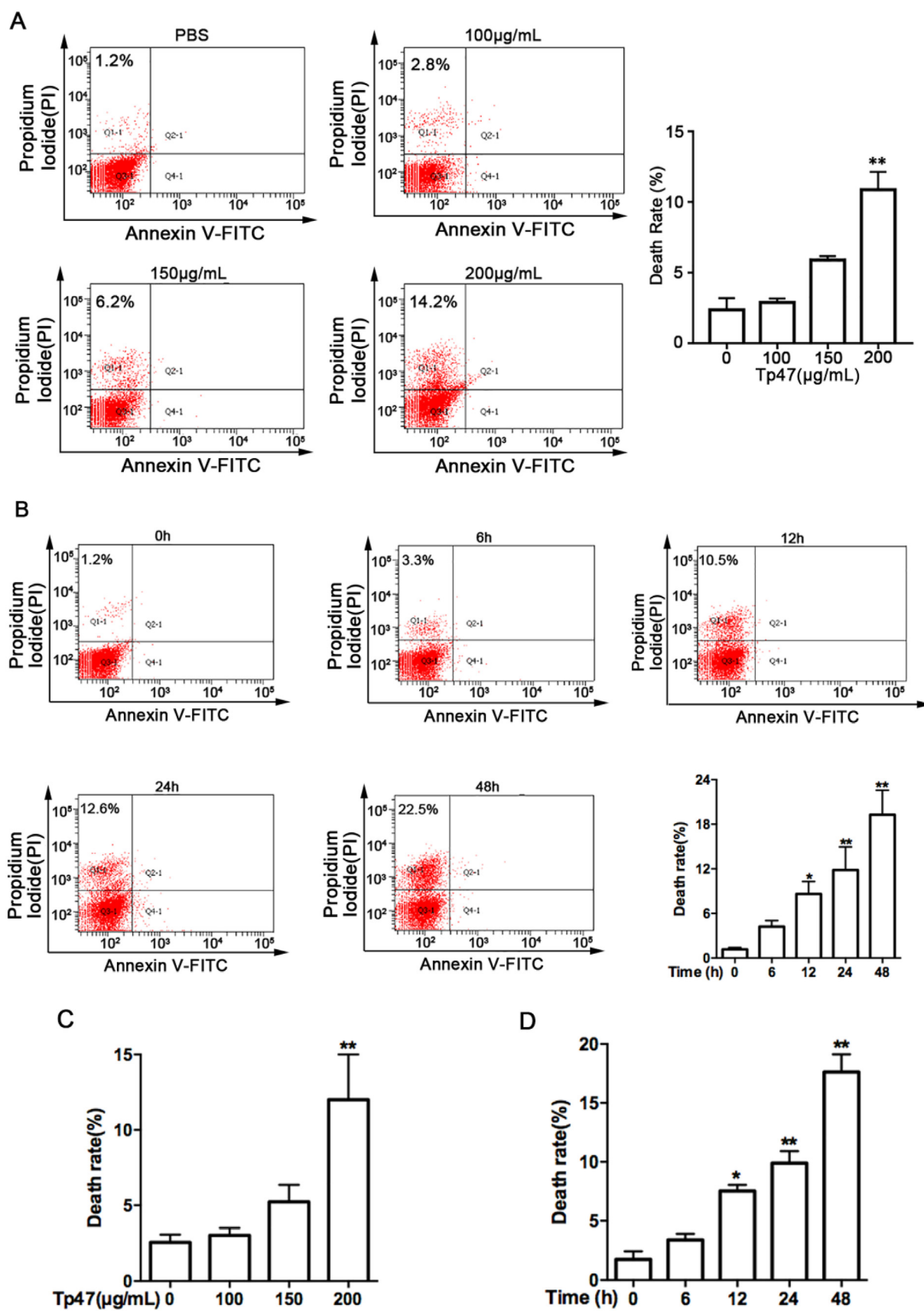
Fig. 2. Tp47 induced HMO6 human microglial cell death in a dose- and time-dependent manner.
