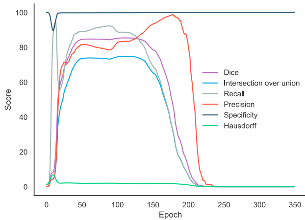
Fig. 6. Per-epoch validation results for the teacher model at center 3 with cross-entropy as the consistency loss. Training was conducted in both centers 1 and 2 simultaneously, and adapted to center 3 with consistency weight \gamma = 5 .
