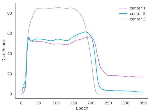
Fig. 7. Per-epoch dice score for the teacher model at center 3 with cross-entropy as the consistency loss. This is an evidence that early stopping can be conducted, although carefully, using data from the source centers. Training was conducted in both centers 1 and 2 simultaneously, and adapted to center 3 with consistency weight \gamma = 5 .
