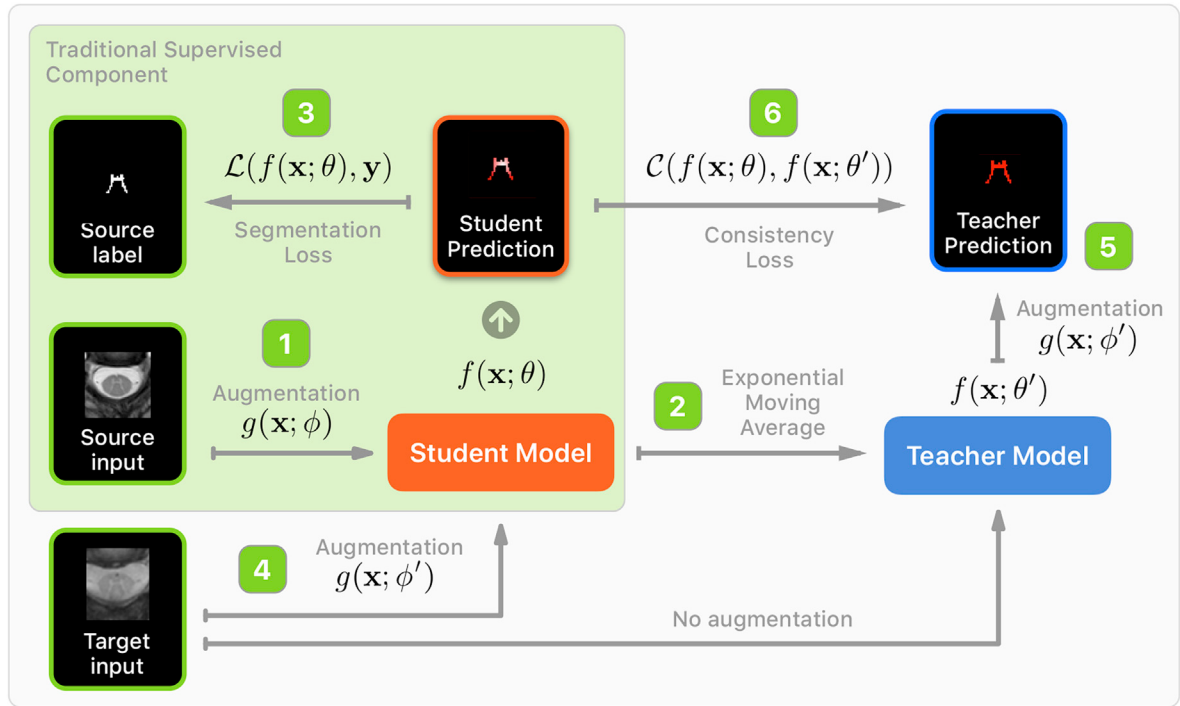
Fig. 4. Overview of the proposed method. The green panel represents the traditional supervision framework. (1) The source domain input slice data is augmented by the g(x; \phi) transformation and fed into the student model. (2) The teacher model parameters is updated with an exponential moving average (EMA) from the student weights. (3) The traditional segmentation loss, where the supervision signal is provided with the source domain labels. (4) The input unlabeled slice data from the target domain is transformed with g(x; \phi') before the student model forward pass (note the different parametrization \phi' ). (5) The teacher model prediction is transformed with g(x; \phi') (same transformation as in Step 4). (6) The consistency loss, which enforces consistency between student and teacher predictions.
