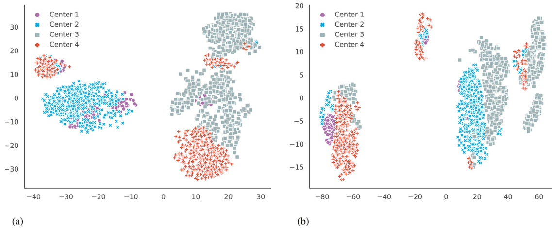
Fig. 8. Execution of t-SNE algorithm for two different scenarios. Colors represent data from different centers. a) A visualization of the t-SNE 2D non-linear embedding projection for the supervised learning scenario. The colors represent data from different centers. b) A visualization of the t-SNE 2D non-linear embedding projection for the domain adaptation scenario. The colors represent data from different centers.
