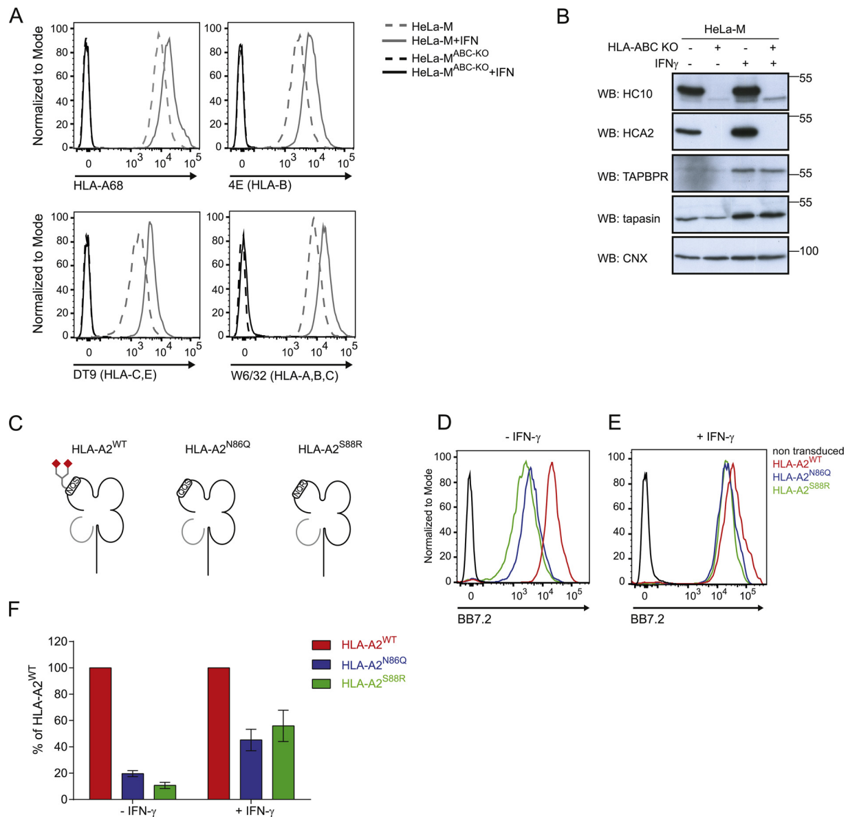
Fig. 3. Glycosylation of N86 is required for efficient surface expression of untaged HLA-A2. (A) Surface expression of HLA-A68, HLA-B (using 4E), HLA-C and -E (using DT9) and pan-MHC class I (detected with W6/32) on HeLa-M (grey line) and HeLa-M ABC-KO cells (black line) treated without (dashed line) and with IFN-γ for 48 h (solid line). (B) Western blot analysis of MHC class I (detected with HC10 and HCA2), TAPBPR, and tapasin on HeLa-M and HeLa-M ABC-KO cells treated without and with IFN-γ for 48 h. Blotting with calnexin is included as a loading control. (C) Cartoon representation of untaged HLA-A2 molecules transduced into the HeLa-M ABC-KO cells. HLA-A2 WT contains the consensus sequence that permits glycosylation of HLA-A2, whereas HLA-A2 N86Q and HLA-A2 S88R are non-glycosylated due to disruption of the motif. (D&E) Surface expression of untaged HLA-A2 detected with the conformational specific mAb BB7.2 on HeLa-M ABC-KO cells expressing HLA-A2 WT (red line), HLA-A2 N86Q (blue line) and HLA-A2 S88R (green line) in (D) the absence and (E) the presence of IFN-γ treatment for 48 h. Staining of non-transduced HeLa-M ABC-KO cells is included as a control (black line). (F) Bar graphs showing mean fluorescence intensity of surface HLA-A2 expression on the panel of HLA-A2 expressing HeLa-M ABC-KO cells as a percentage of HLA-A2 WT . Error bars represent SEM from three independent experiments as performed in D & E. (For interpretation of the references to color in this figure legend, the reader is referred to the web version of this article.)
