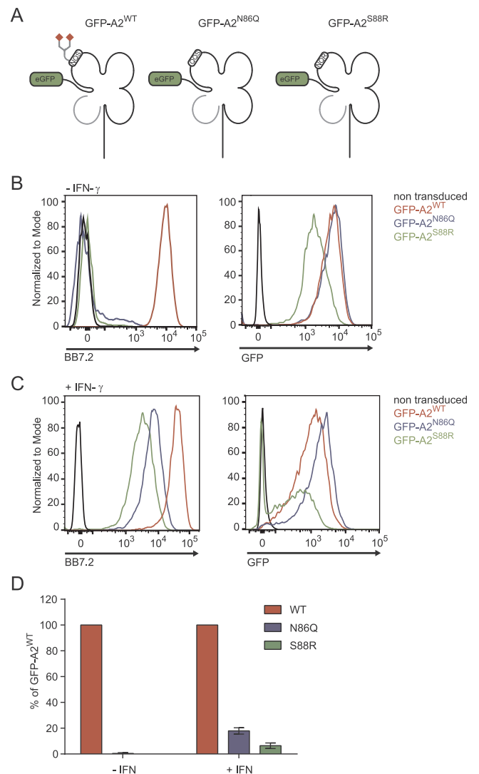
Fig. 1. The N-linked glycan on MHC class I is required for efficient surface expression of GFP-A2. (A) Cartoon representation of the N-terminally GFP tagged HLA-A2 molecules used in this study. GFP-A2 WT contains the consensus sequence that permits glycosylation of HLA-A2, whereas GFP-A2 N86Q and GFP-A2 S88R are non-glycosylated due to disruption of the motif. (B & C) Surface expression of GFP-A2 detected with the conformational specific mAb BB7.2 and total GFP expression to demonstrate transduction efficiency in HeLa-M cells expressing GFP-A2 WT (red line), GFP-A2 N86Q (blue line) and GFP-A2 S88R (green line) in (B) the absence and (C) the presence of IFN- \gamma treatment for 48 h. Staining of non-transduced HeLa-M cell with BB7.2 is included as a control (black line). The results are representative of three independent experiments. (D) Bar graphs showing mean fluorescence intensity of surface HLA-A2 expression on the panel of GFP-A2 expressing cell lines as a percentage of GFP-A2 WT . Error bars represent SEM from three independent experiments as performed in B & C. (For interpretation of the references to color in this figure legend, the reader is referred to the web version of this article.)
