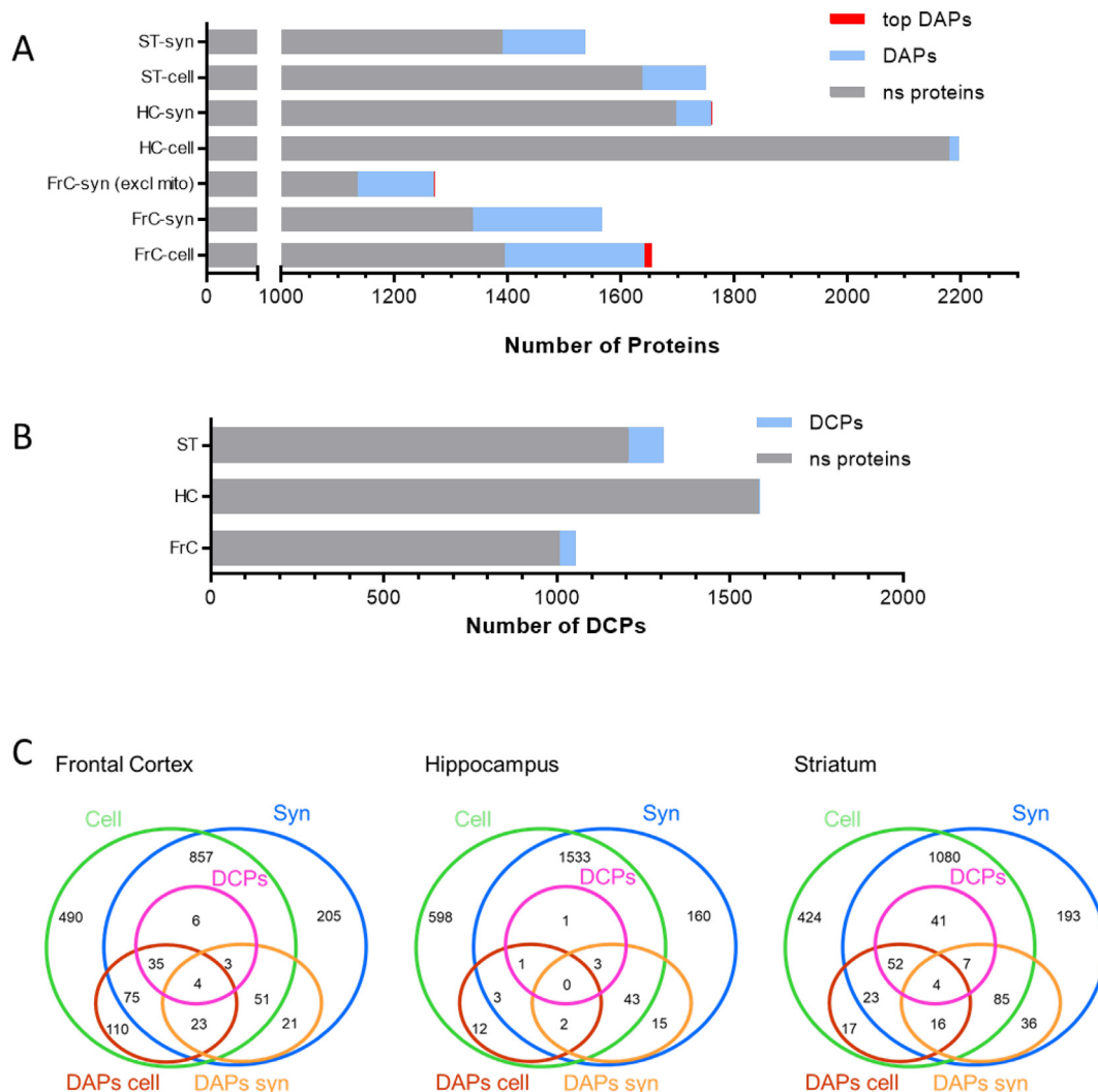
Fig. 2. A) Total number of unique proteins detected in female Brd1 +/- mouse brain regions. Differentially abundant proteins (DAPs, p < .05 and LFC > \text{cut-off} ); top differentially abundant proteins (Top DAPs p < .001 and LFC > \text{cut-off} ). LFC cut-off: \pm 0.231 (FrC-Cell), \pm 0.104 (FrC-Syn), \pm 0.099 (FrC-Syn (excl mito)), \pm 0.191 (HC-Cell), \pm 0.072 (HC-Syn), \pm 0.189 (ST-Cell), \pm 0.102 (ST-Syn). B) Total number of unique proteins shared between cell lysate and synaptosomal preparations of the same brain region and differentially compartmentalized proteins (DCPs, p < .05 ). C) Distribution of the proteins among fractions and statistical significant groups. Abbreviations: frontal cortex (FrC); hippocampus (HC); striatum (ST); cell lysate (cell); synaptosome (syn); not significant (ns).
