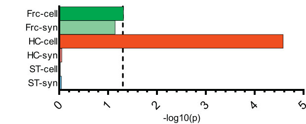
Fig. 3. MAGMA disease risk enrichment analysis for schizophrenia. Black dashed line: significance threshold ( p = .05 ). Abbreviations: frontal cortex (Frc); hippocampus (HC); striatum (ST); cell lysate (cell); synaptosome (syn).
