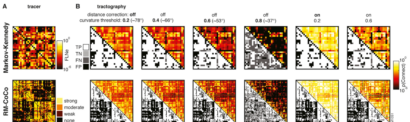
Fig. 1. (A) Tracer-derived connectivity matrices from Markov et al. (2014) (top) and CoCoMac ( Shen et al., 2012 ; Stephan et al., 2001 ) (bottom). (B) Tractography-derived matrices (upper triangle) for an example subject for each parcellation (Markov-Kennedy, top; RM-CoCo, bottom) using various tractography parameters. Accuracy of each connection, as compared to tracer-derived matrices, depicted in lower triangles (TP: true positive; TN: true negative; FN: false negative; FP: false positive). For the RM-CoCo parcellation, left hemisphere ROIs are ordered together followed by right hemisphere ROIs, such that interhemispheric quadrants are the upper right and lower left of each matrix.
