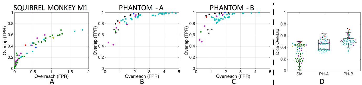
Fig. 4. Voxel-wise spatial overlap validation. Plots of overlap versus overreach are shown for the squirrel monkey (A) and phantom datasets on scanner A (B) and scanner B (C). Boxplots of the corresponding Dice overlap coefficients are shown for both challenges (D). One marker is shown per submission, with marker colors indicating unique research groups.
