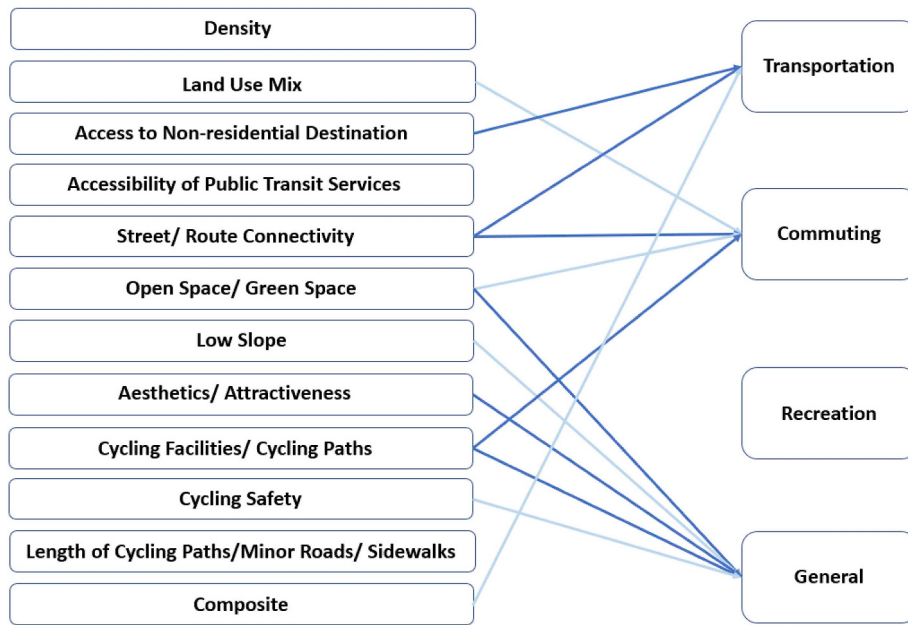
Fig. 2. The strengths of associations between built environmental factors and different cycling purpose. Strong associations (the number of expected results was greater than twice the sum of unexpected and null results) are shown as dark blue lines. Emerging associations (where the number of expected results was more than the sum of unexpected and null results but less than twice of the sum) are shown as light blue lines. (For interpretation of the references to color in this figure legend, the reader is referred to the Web version of this article.)
