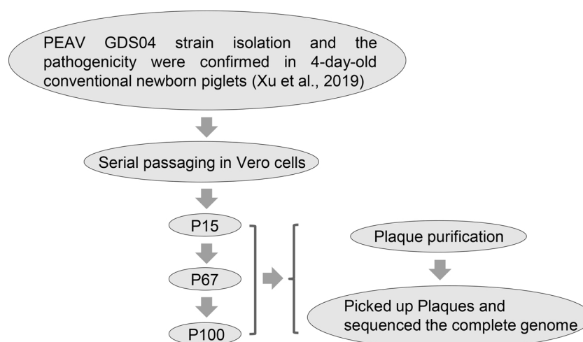
Fig. 1. The flowchart of the isolation and passing of PEAV GDS04 strain in Vero cells.
