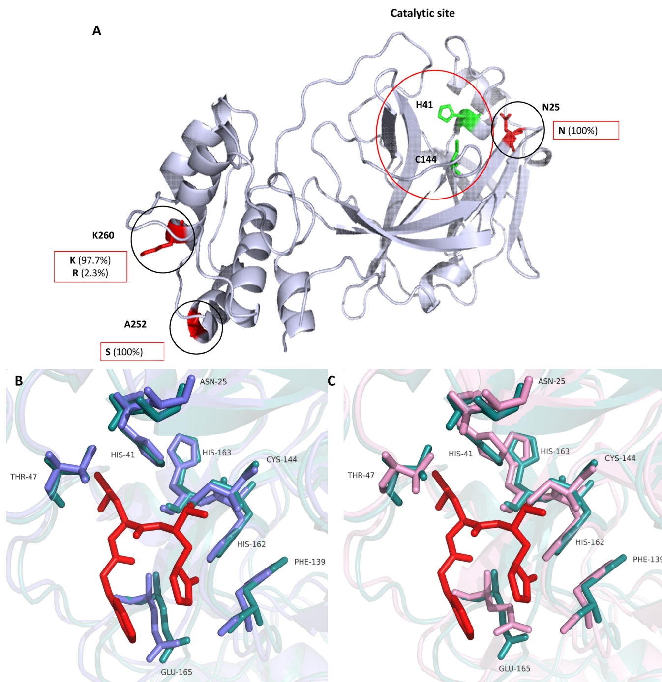
Fig. 4. The structure of feline coronavirus 3CLpro and amino acid substitutions. (A) A ribbon representation of a feline coronavirus 3CLpro (PDB accession: 4ZRO) was prepared using the PyMol program. The catalytic residues (H41 and C144) are shown in green, and N25, A252 and K260 are shown in red. The amino acids found at the position of 25, 252 and 260 in 3CLpro among feline coronavirus strains whose 3CLpro amino acid sequence are available in the PubMed database are shown in red boxes. (B) Active site of the superimposed crystal structures of TGEV 3CLpro-GC376 (PDB accession: 4F49) (teal) and feline coronavirus 3CLpro (PDB accession: 4ZRO) (slate). (C) Active site of the superimposed crystal structure of TGEV 3CLpro-GC376 (PDB accession: 4F49) (teal) and a homology model of CT10 WT 3CLpro (pink). GC376 (red) is shown as a red stick (For interpretation of the references to colour in this figure legend, the reader is referred to the web version of this article).
