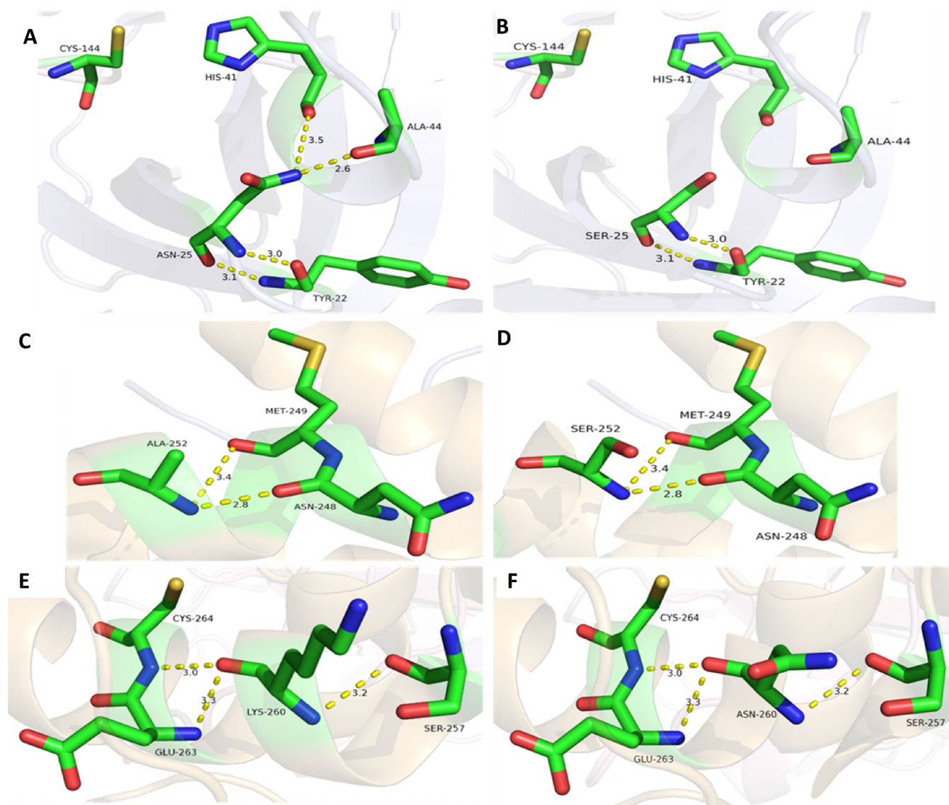
Fig. 5. The effects of amino acid changes on the putative hydrogen bond formation by N25, A252 and K260 in feline coronavirus 3CLpro. The active site of wild type 3CLpro with predicted hydrogen bonds are shown in panels A, C and E. (A and B) The N25S substitution is predicted to result in the loss of hydrogen bonds (dashed lines) formed between N25 and H41 and A44, but not with Y22. (C to F) The A252S (C and D) and K260N (E and F) substitutions are not predicted to affect the hydrogen bonds. The hydrogen bonds between N25 (A), A252 (C) and K260 (E) with neighboring amino acids in feline coronavirus 3CLpro are shown with the distance measurements in Å.
