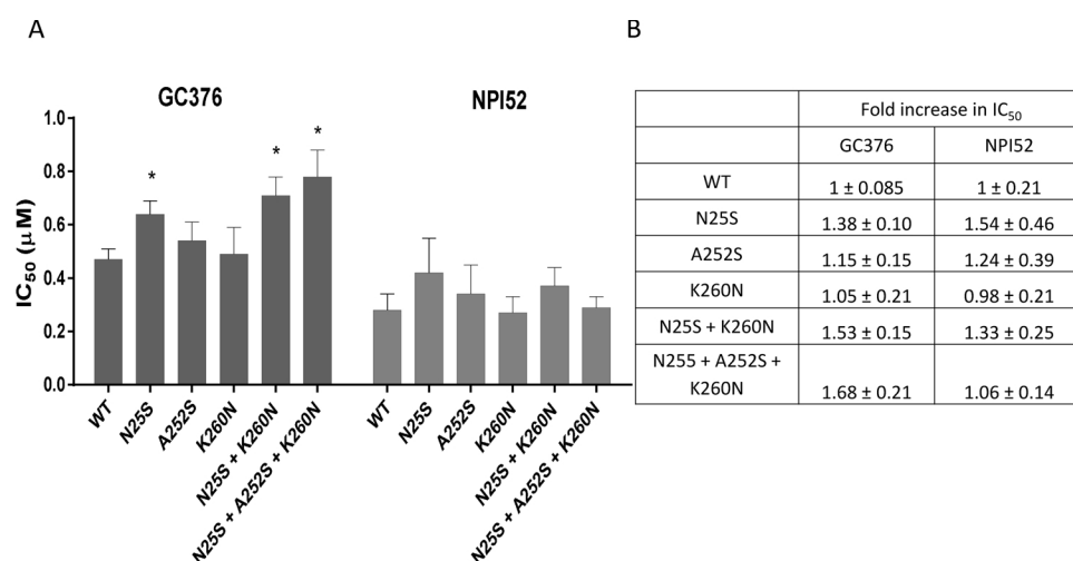
Fig. 3. Effects of GC376 and NPI52 on recombinant wild-type and mutant 3CLpros in the FRET assay. Each 3CLpro was incubated with serial dilutions of GC376 or NPI52 for 30 min at 37 °C, and then fluorogenic substrate was added to the mixture. Following incubation for 30 min, fluorescence readings were measured on a fluorescence microplate reader for the determination of IC 50 values. (A) Each bar represents the mean ± standard error of the means from at least three independent FRET assays. (B) Fold increases in IC 50 values of mutant 3CLpro over those of WT 3CLpro are shown in the table. WT indicates wild-type (pre-treatment) 3CLpro. N25S, A252S and K260 N indicates 3CLpros carrying a single mutation. N25S + K260 N and N25S + A252S + K260 N indicate double and triple mutations, respectively. Asterisks indicate statistically significant difference compared to WT ( P < 0.05 ).
