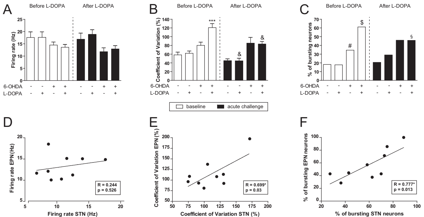
Fig. 2. Electrophysiological characterization of the Entopeduncular nucleus, and regression analysis between STN neurons and EPN neurons electrophysiological parameters recorded in the same rat. (A) Firing rate (Hz) of EPN GABAergic neurons. Baseline firing rate (white bars) was not significantly different in the four experimental groups. The acute challenge of L-DOPA (6 mg/kg, i.p.) plus benserazide (12 mg/kg i.p.) (black bars) did not modify the firing rate in the different experimental groups. (B) Coefficient of variation (%). Baseline activity (white bars) was significantly increased in 6-OHDA L-DOPA group. The acute challenge of L-DOPA plus benserazide produced a significant reduction in sham L-DOPA and 6-OHDA L-DOPA groups. (C) Firing pattern of EPN cells expressed as percentage of neurons. Baseline bursting firing pattern (white bars) was significantly increased in 6-OHDA lesioned groups. After the acute challenge of L-DOPA plus benserazide, the number of bursting neurons was reduced in the 6-OHDA L-DOPA group. (D) Pearson r value for the correlation between the firing rate of STN neurons and EPN neurons recorded 24 h after the last L-DOPA injection in the same long term L-DOPA treated 6-OHDA-lesioned rats. (E) Pearson r value for the correlation between the coefficient of variation of STN neurons and EPN neurons recorded 24 h after the last L-DOPA injection in the same long term L-DOPA treated 6-OHDA-lesioned rats. (F) Pearson r value for the correlation between the percentage of bursting neurons of STN neurons and EPN neurons recorded 24 h after the last L-DOPA injection in the same long term L-DOPA treated 6-OHDA-lesioned rats. Data are expressed as mean \pm S.E.M. *** p < .001 vs. sham saline and sham L-DOPA (Bonferroni's post-hoc test); * p < .05 vs. its baseline (unpaired t -test); # p < .05 vs. sham L-DOPA (Fisher's exact-test for firing pattern); $ p < .05 vs. sham saline, sham L-DOPA and 6-OHDA saline (Fisher's exact-test for firing pattern); § p < .05 vs. its baseline (Fisher's exact-test for firing pattern); * p < .05 (Pearson r value).
