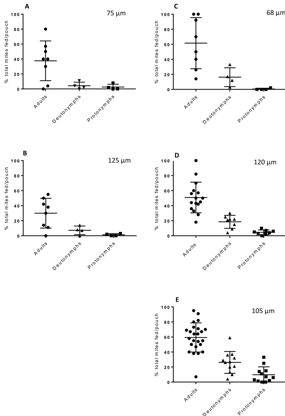
Fig. 2. The ability of hematophagous life stages of Dermanyssus gallinae to take a blood meal from hens through nylon meshes with aperture dimensions of 75 \mu\text{m} wide by 150 \mu\text{m} deep (Panel A) and 125 \mu\text{m} wide by 170 \mu\text{m} deep (Panel B) and polyester mesh with aperture dimensions of 68 \mu\text{m} by 45 \mu\text{m} deep (Panel C), nylon mesh with aperture dimensions of 120 \mu\text{m} by 82 \mu\text{m} deep (Panel D) and polyester mesh with aperture dimensions of 105 \mu\text{m} by 63 \mu\text{m} deep (Panel E). Means are shown ( \pm SEM) and mesh aperture size shown in the top right hand corner of each panel.
