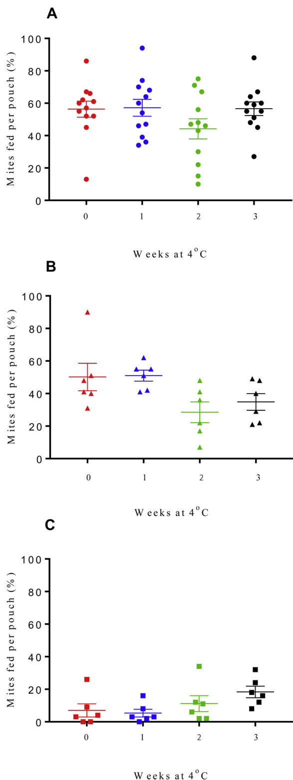
Fig. 3. Feeding success of hematophagous life stages of Dermanyssus gallinae feeding on hens through a polyester mesh with aperture dimensions of 105 \mu m wide by 63 \mu m deep after different starvation protocols (“Weeks at 4 °C”). Panel A shows data for adult mites; Panel B deutonymphs and Panel C protonymphs. Means are shown ( \pm SEM).
