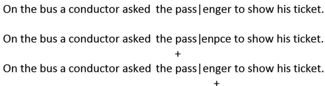
Fig. 2. The + sign shows the location of the eye during a fixation on the line above the +. The vertical line shows the location of the invisible boundary.
