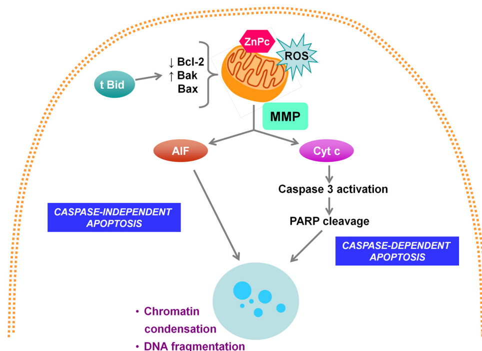
Fig. 3. Mitochondria membrane permeabilization (MMP) induced by deregulation in the expression levels of Bcl-2 family proteins leads to activation of either caspase- dependent and independent apoptosis.
