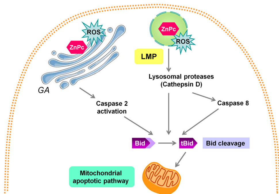
Fig. 4. Contribution of GA photodamage and lysosomal membrane permeabilization (LMP) to the activation of the mitochondrial-dependent apoptosis.
