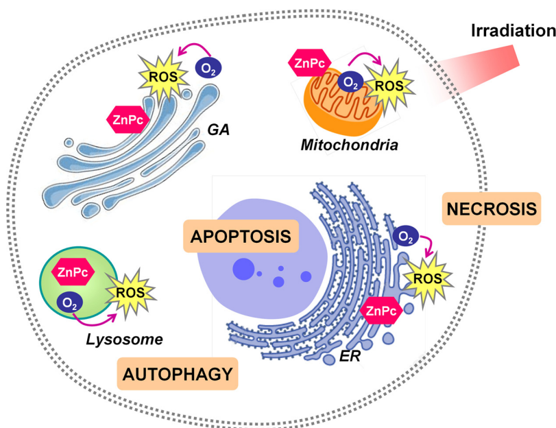
Fig. 2. Main intracellular sites of ZnPcs localization. After irradiation, ZnPcs promote the generation of ROS that triggers different phototoxic cellular responses.
