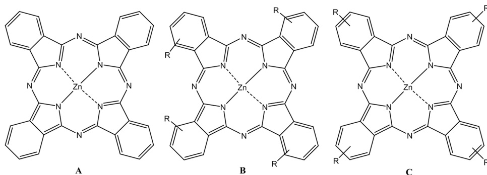
Fig. 1. Chemical structure of ZnPc (A), \alpha -tetrasubstituted ZnPc (B) and \beta -tetrasubstituted ZnPc (C).
