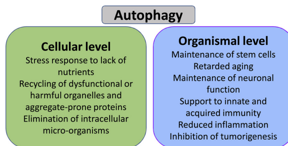
Fig. 5. Summary of the functions of autophagy at cellular and organismal levels.
