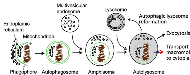
Fig. 2. Schematic drawing of the macroautophagy pathway. Phagophores emerge between two endoplasmic reticulum cisternae, and close to form autophagosomes. Autophagosomes fuse with endosomes and lysosomes to mature into autolysosomes, which are the main degradative compartment of the pathway. Lysosomes can reform from autolysosomes, and autolysosomes can also fuse with the plasma membrane and empty their contents to the extracellular space.
