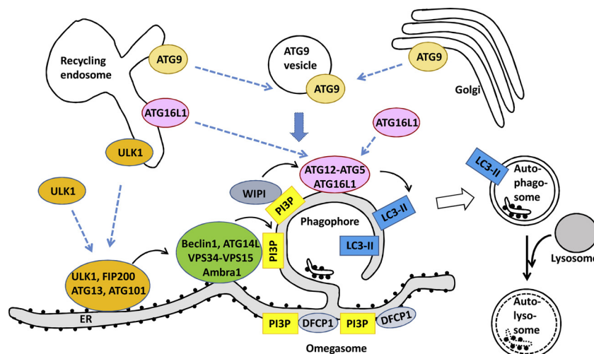
Fig. 3. Overview of proteins, protein complexes and organelles that participate in autophagosome formation. See text for further details.
