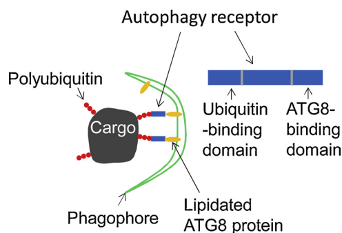
Fig. 4. Schematic drawing of ubiquitin-dependent selective autophagy. Note that part of the autophagy receptors are independent of cargo ubiquitination.
