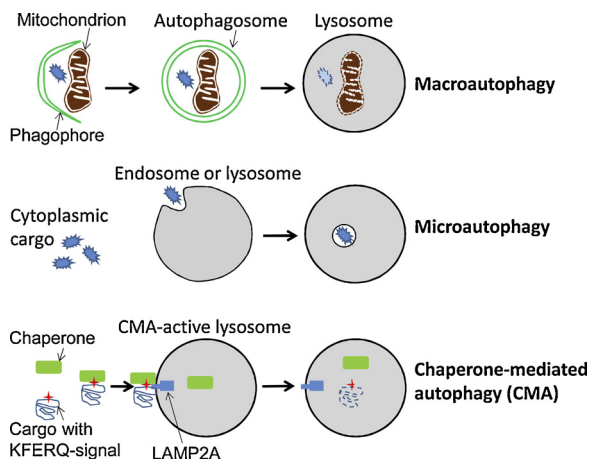
Fig. 1. Schematic representation of the three autophagic pathways that deliver cargo from cytoplasm to lysosomes.
